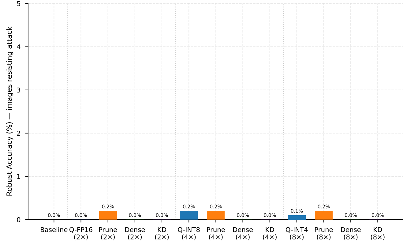
LaVAN Untargeted — Side-8 (6.25% area)
