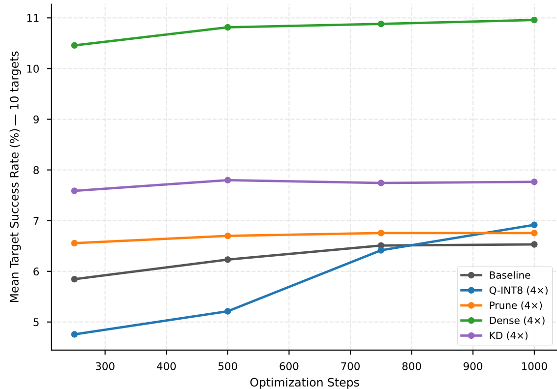
Attack Convergence — Side-5
