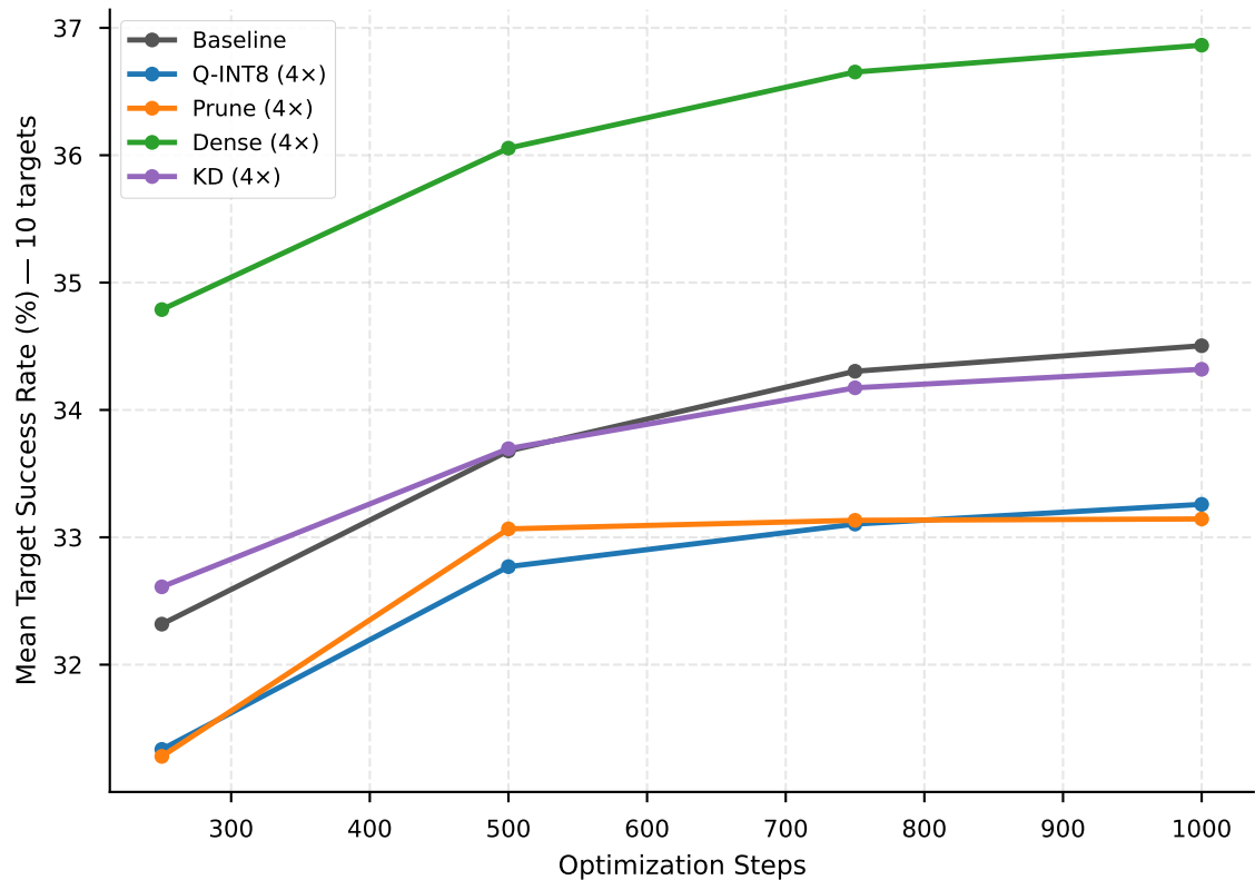
Attack Convergence — Side-8
