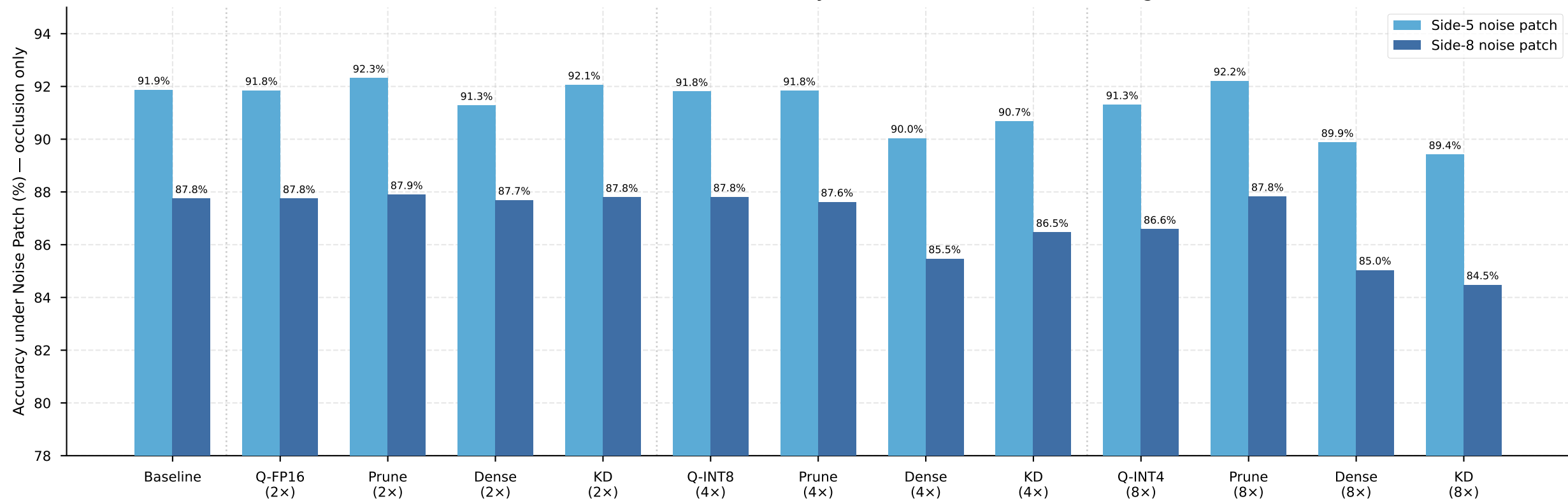
Occlusion Baseline: Noise-Patch Accuracy (Random Patch, No Adversarial Signal)
