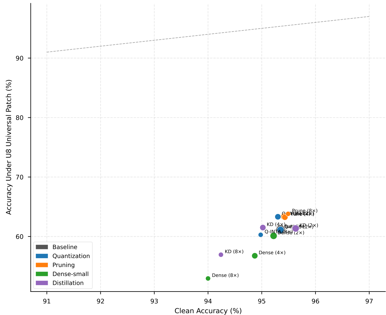
Clean vs. Adversarial Robustness Trade-off
