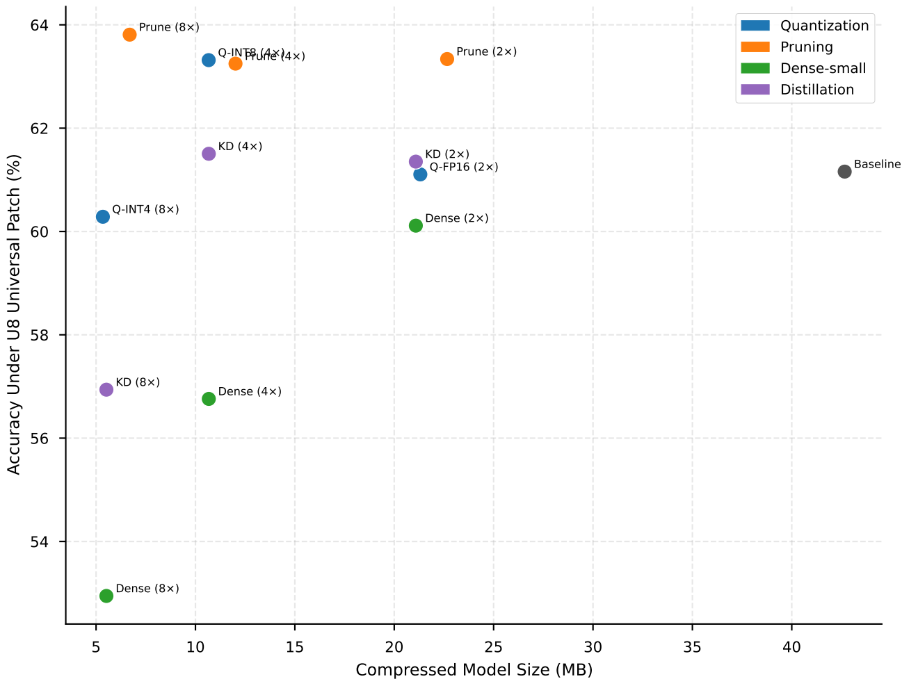
Model Size vs. Universal-Patch Robustness
