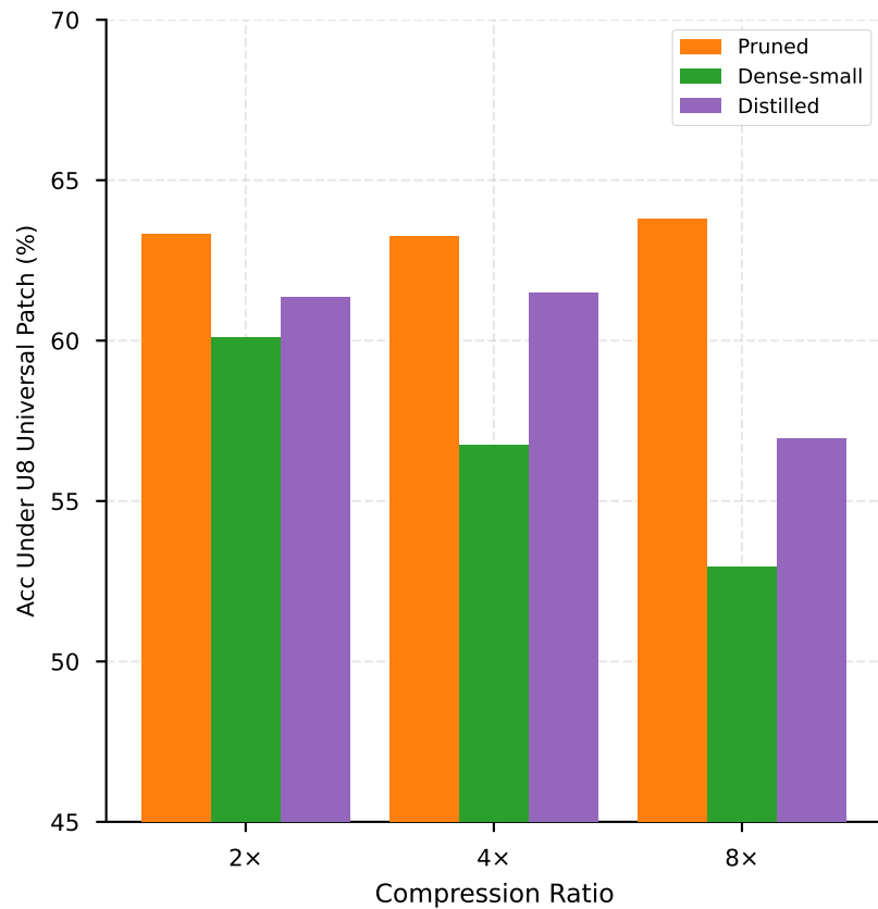
RQ4: Sparsity vs. Capacity — Pruned vs. Dense-small vs. Distilled (Matched nonzero parameters at each ratio)
