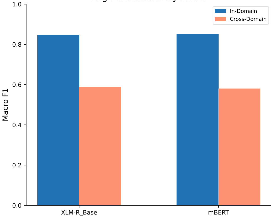
Avg Performance by Model
