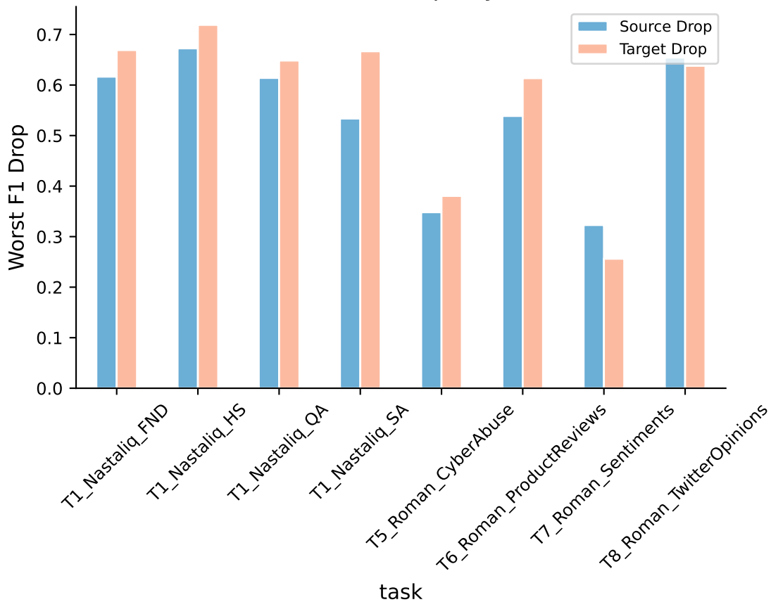
Worst-Case Drops by Task
