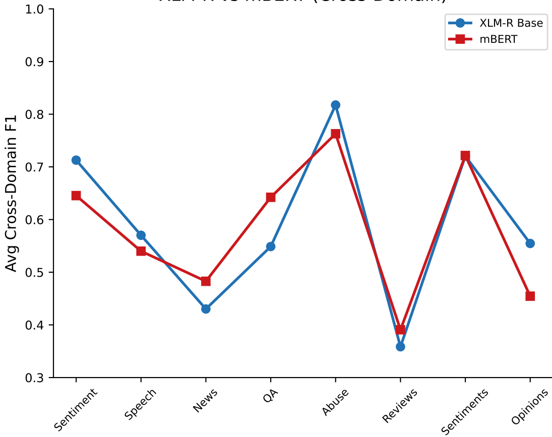
XLM-R vs mBERT (Cross-Domain)
