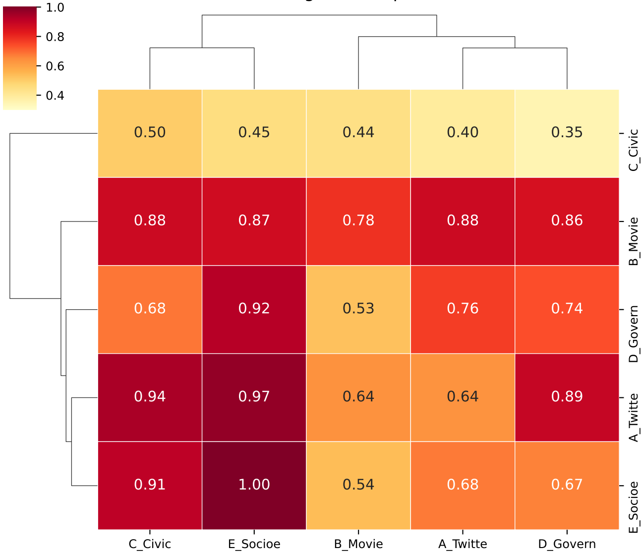
Domain Clustering: Nastaliq Sentiment
