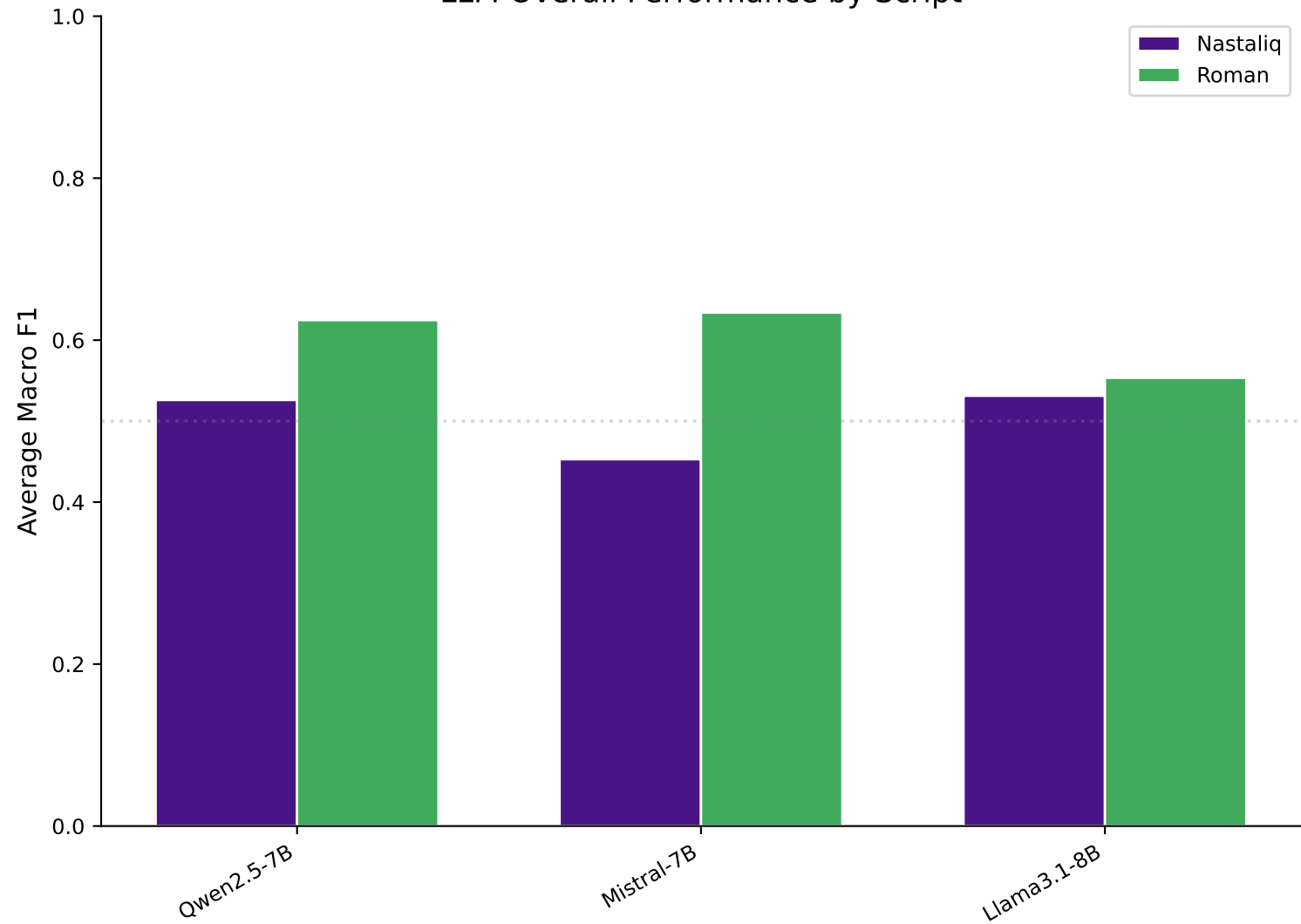
LLM Overall Performance by Script
