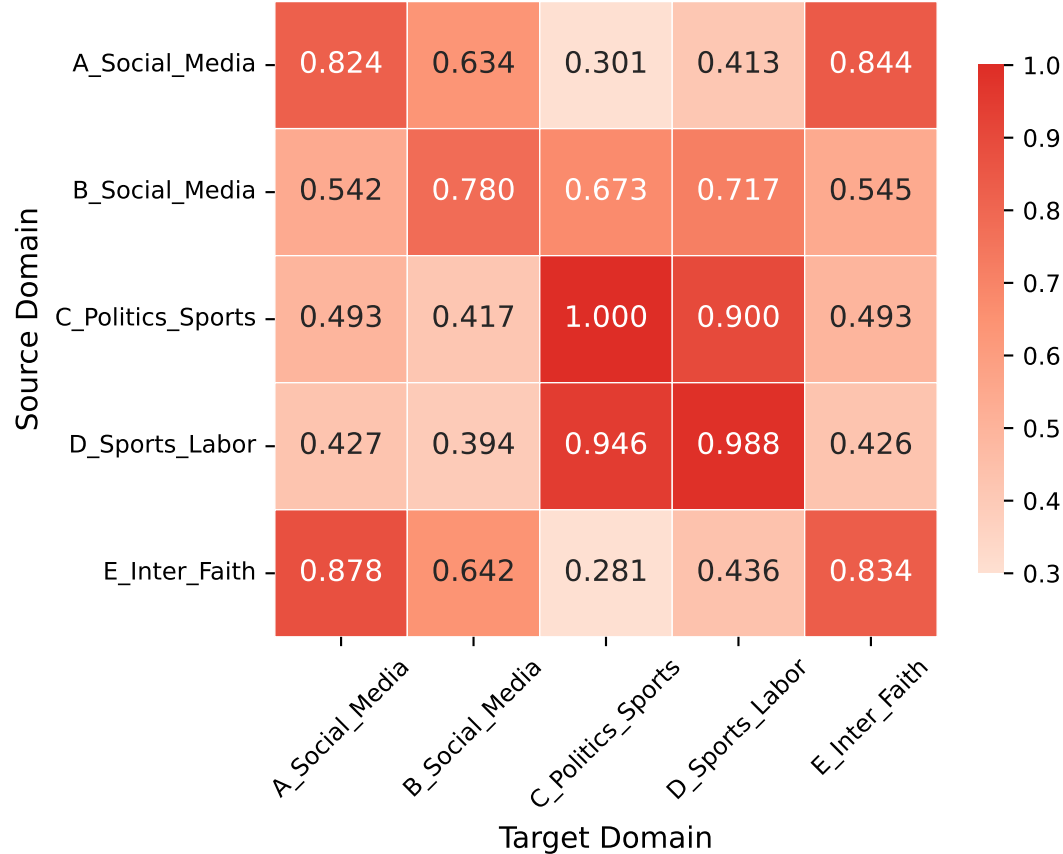
Cross-Domain F1 Performance Matrix: Nastaliq Hate Speech (XLM-R Base)
