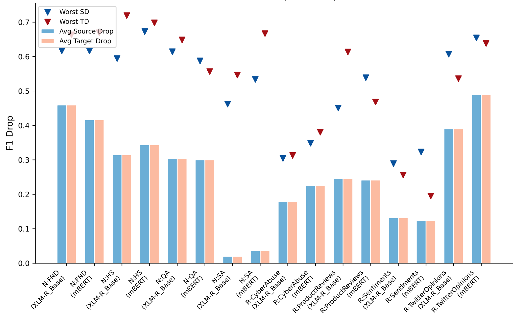
Domain Shift Impact (Drops)
