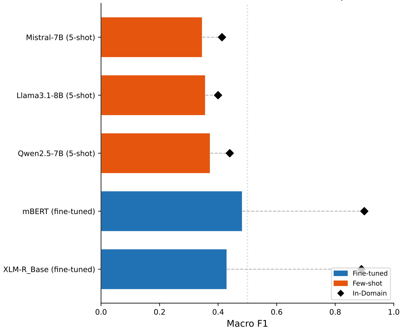
Fine-Tuned vs Few-Shot LLM: T1 Nastaliq FND
