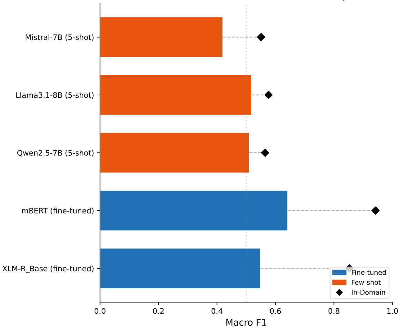
Fine-Tuned vs Few-Shot LLM: T1 Nastaliq QA
