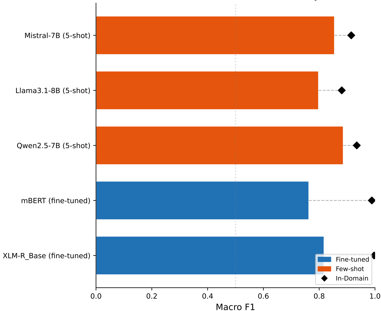
Fine-Tuned vs Few-Shot LLM: T5 Roman CyberAbuse
