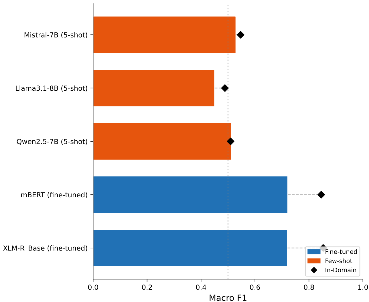
Fine-Tuned vs Few-Shot LLM: T7 Roman Sentiments
