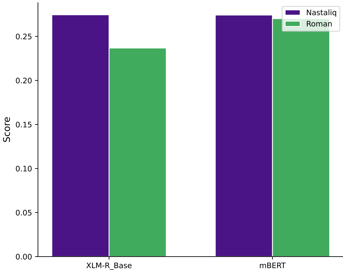
Script Comparison: Avg Source Drop
