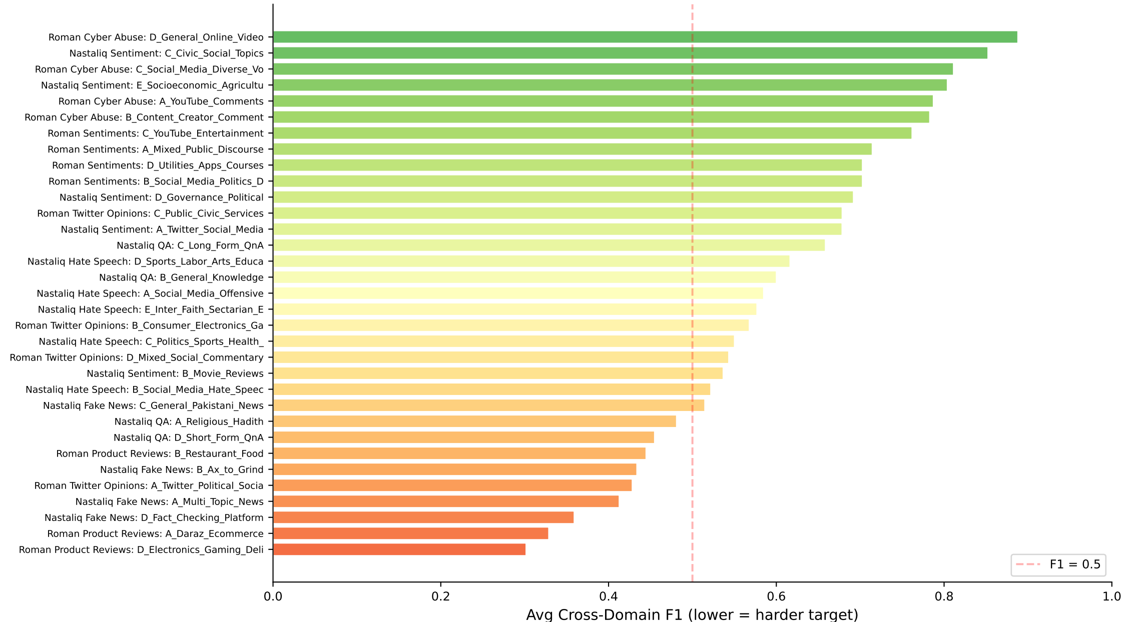
Domain Difficulty Ranking (as Transfer Target)
