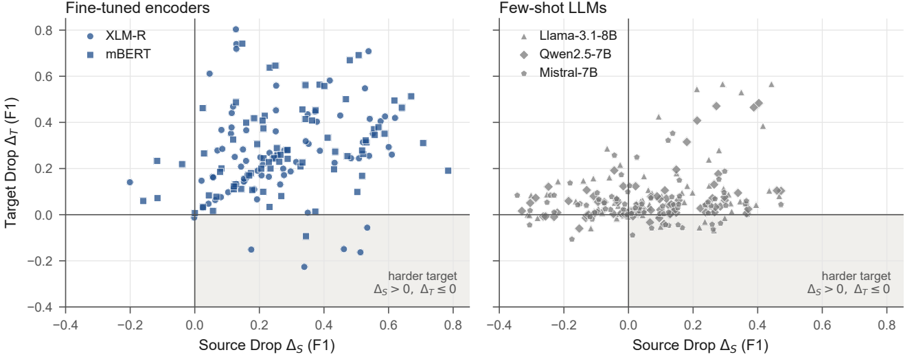
Figure 5. Source Drop against Target Drop for every shift (one point per shift and model, means over seeds). Points in the shaded lower-right region are harder-target shifts: the source model loses performance but matches or beats the target’s own model.
