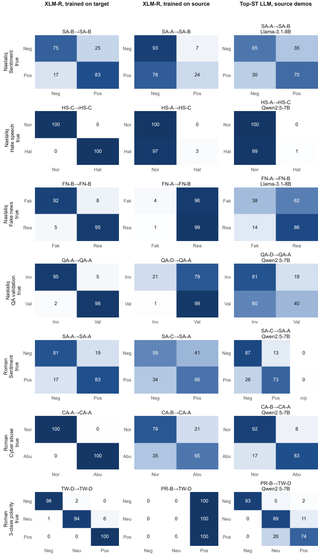
Figure 7. Confusion matrices (row-normalised, %, summed over three seeds) for the worst-transferring shift of each matrix. Left: XLM-R trained on the target (in-domain reference). Middle: XLM-R trained on the source. Right: the few-shot LLM with the highest mean ST in the matrix, prompted with source demonstrations, on its evaluation sample; n/p = unparseable output. Darker cells hold more items.
