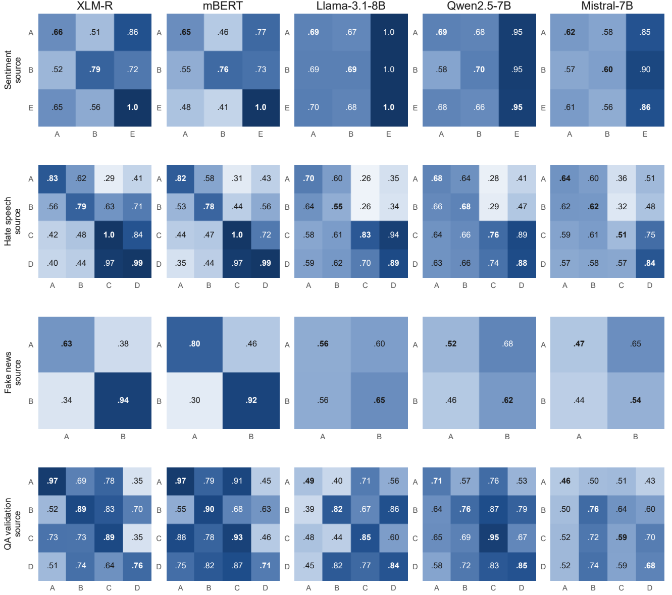
Figure 3. Nastaliq transfer matrices: macro-F1 of a model trained or prompted on the row domain and tested on the column domain, mean over three seeds or demonstration draws. The diagonal (bold) is in-domain performance; darker cells are higher.
