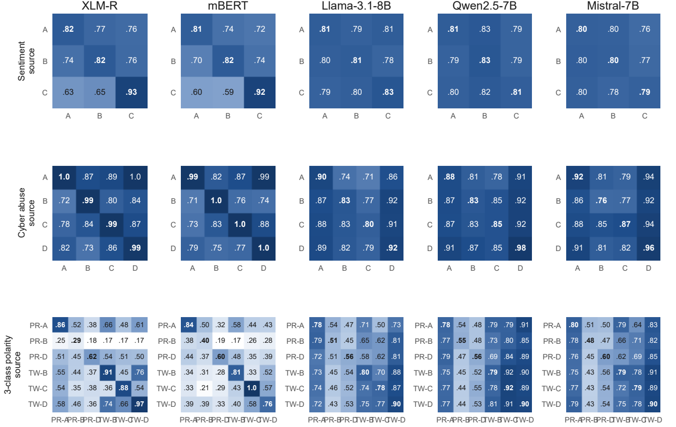
Figure 4. Roman Urdu transfer matrices; layout as in Figure 3.
