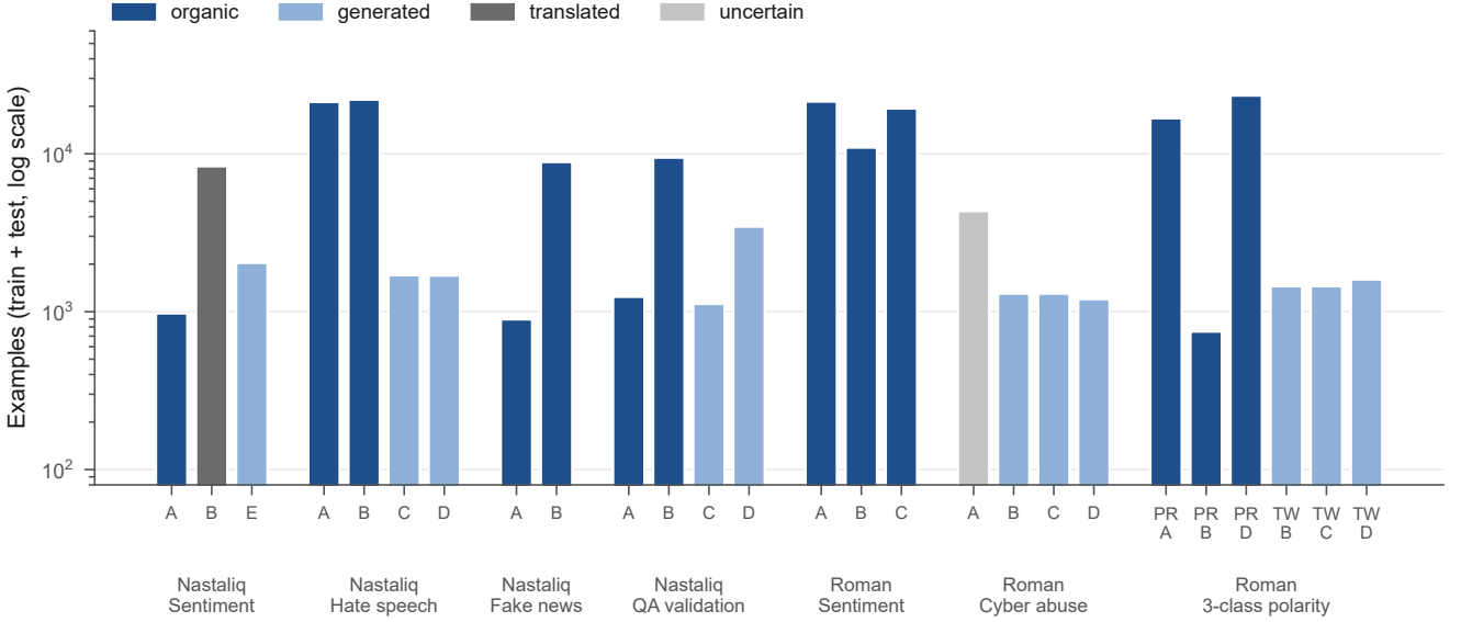
Figure 1. Size of every domain (training and test items, log scale), grouped by transfer matrix and coloured by data origin. Exact counts and class distributions are in Table 2.
