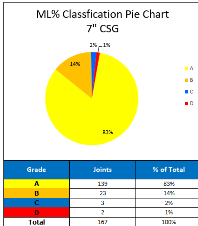
Figure 14 - Metal Loss Pie Chart Summary
