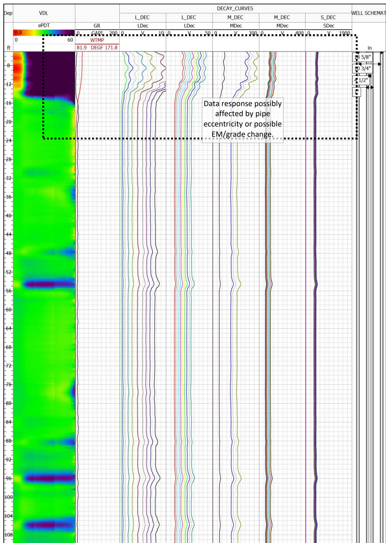
Figure 4 –Well-Head-section
