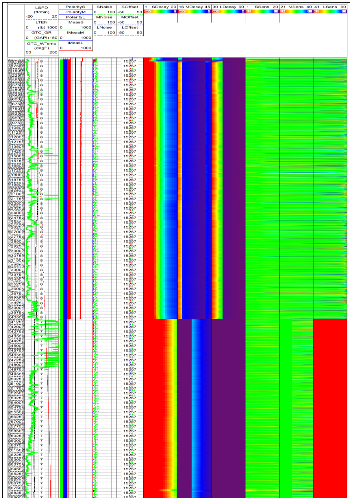
Figure 16 - Main Pass Quality Control
