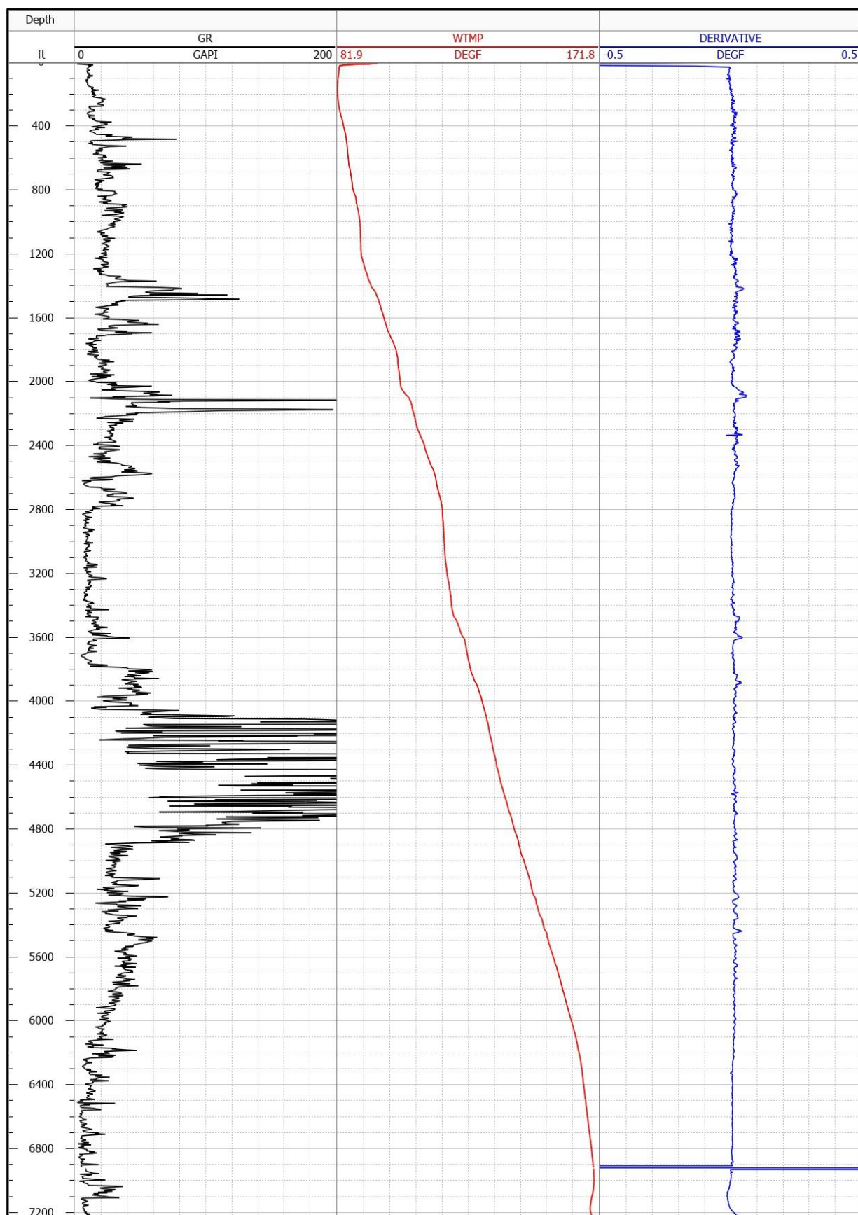
Figure 3 - Expanded Temperature and GR Log
