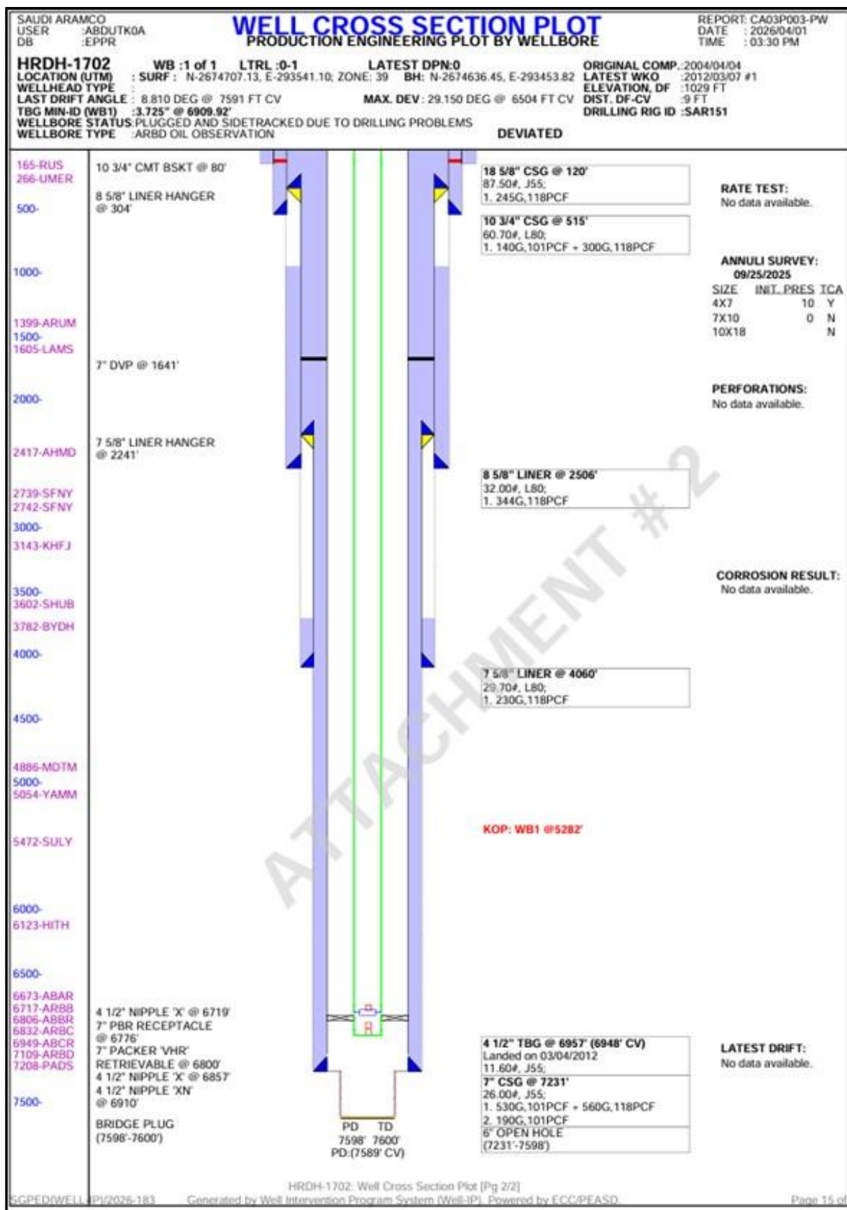
Figure 17 - Well Cross Section Plot
