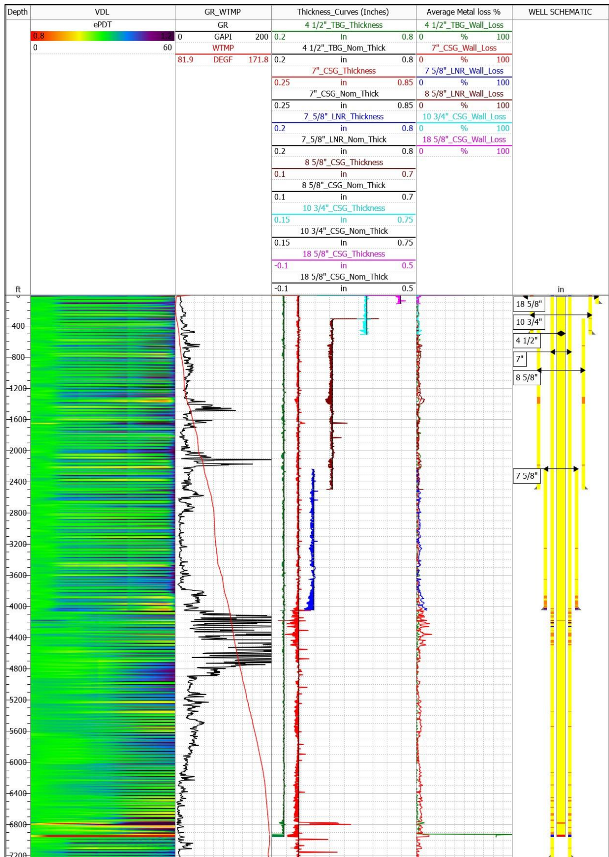
Figure 2 - Four Barriers Metal Loss Evaluation Results
