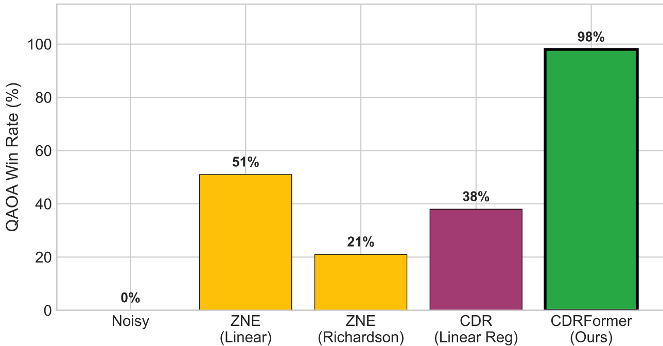
CDRFormer vs Baseline Methods on QAOA Circuits
