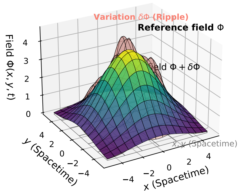
Field Theory: Field over Spacetime
