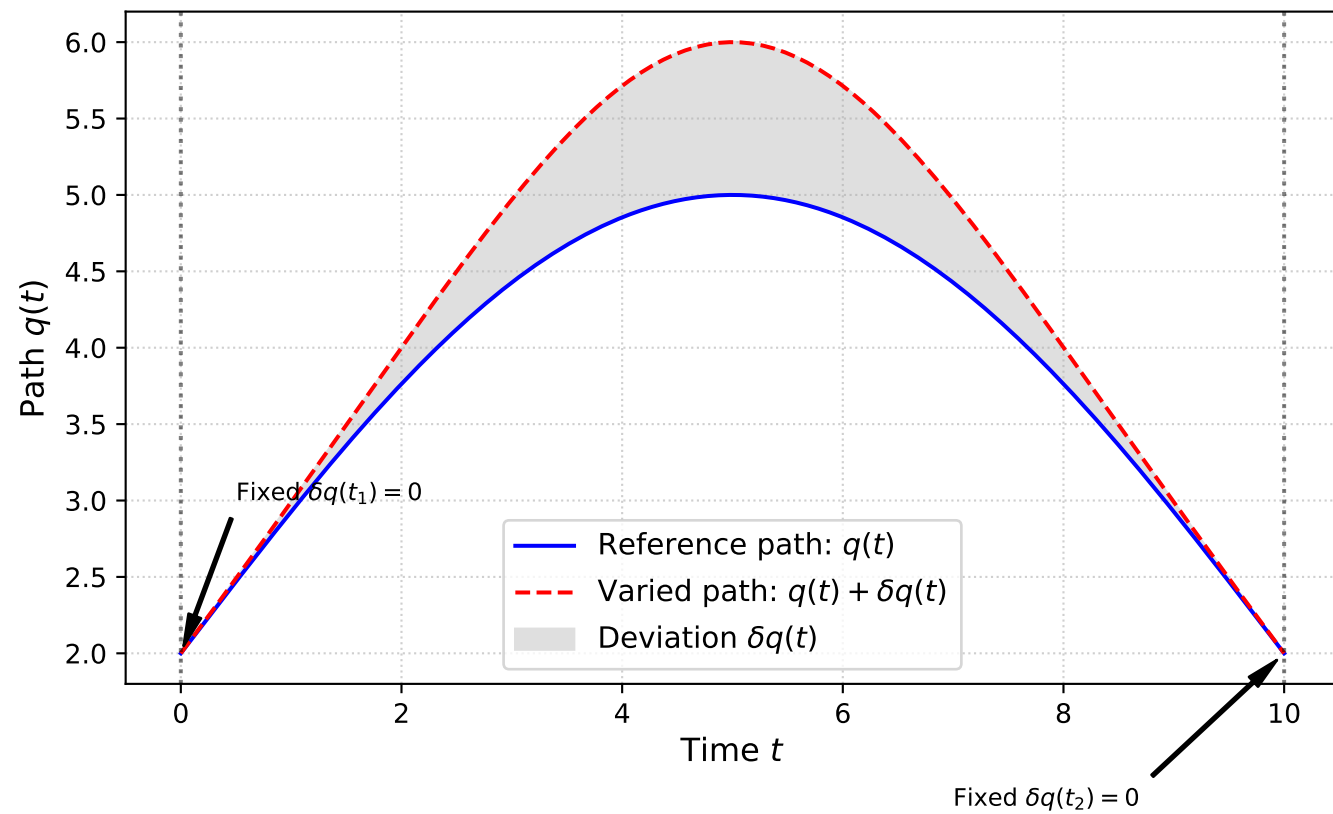
Mechanics: Point Particle Path
