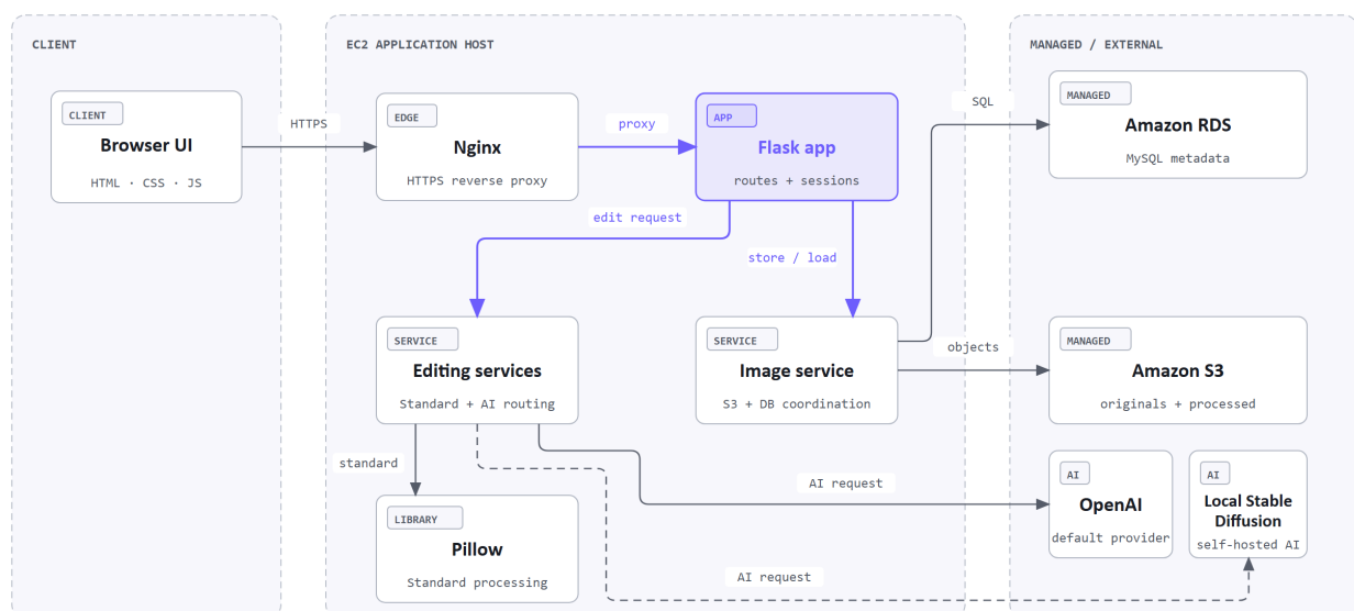
Figure 4.2: NeuroPix system architecture.
