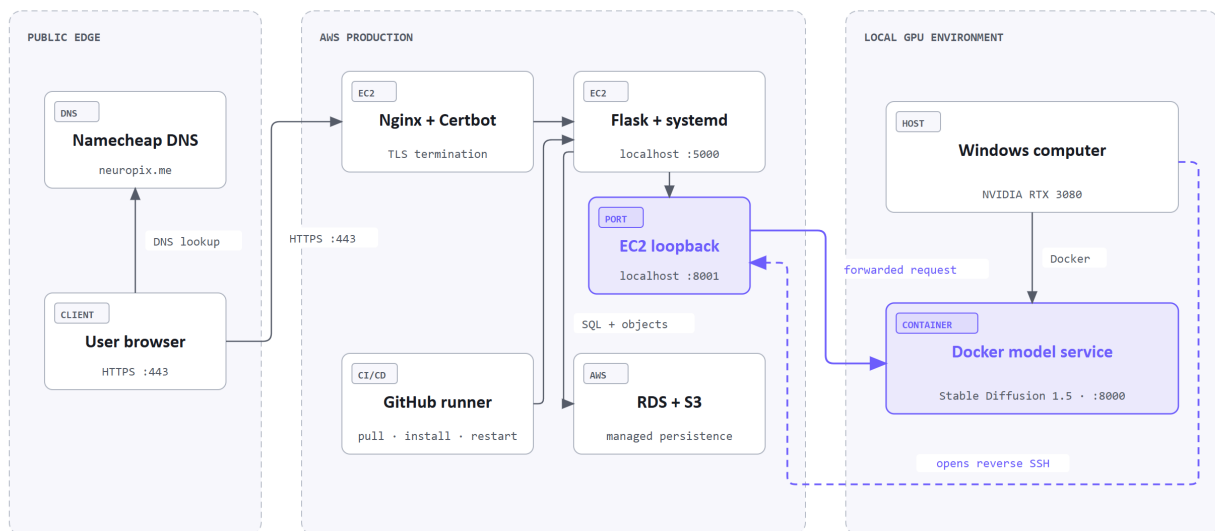
Figure 4.11: Production deployment and reverse SSH.
