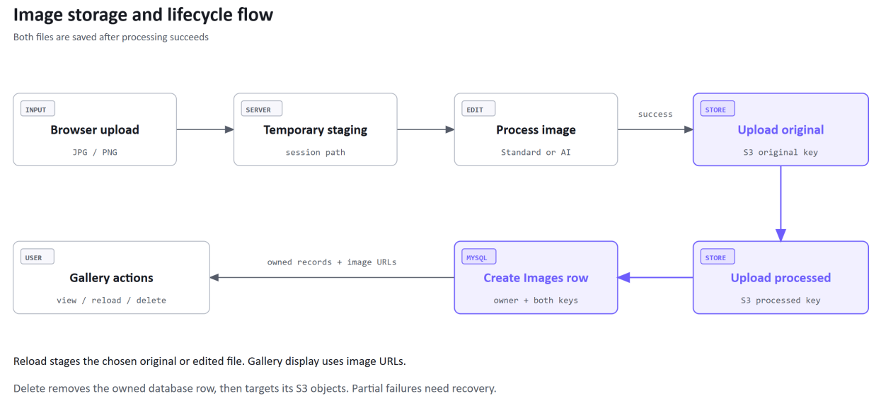
Figure 4.8: Image storage lifecycle.
