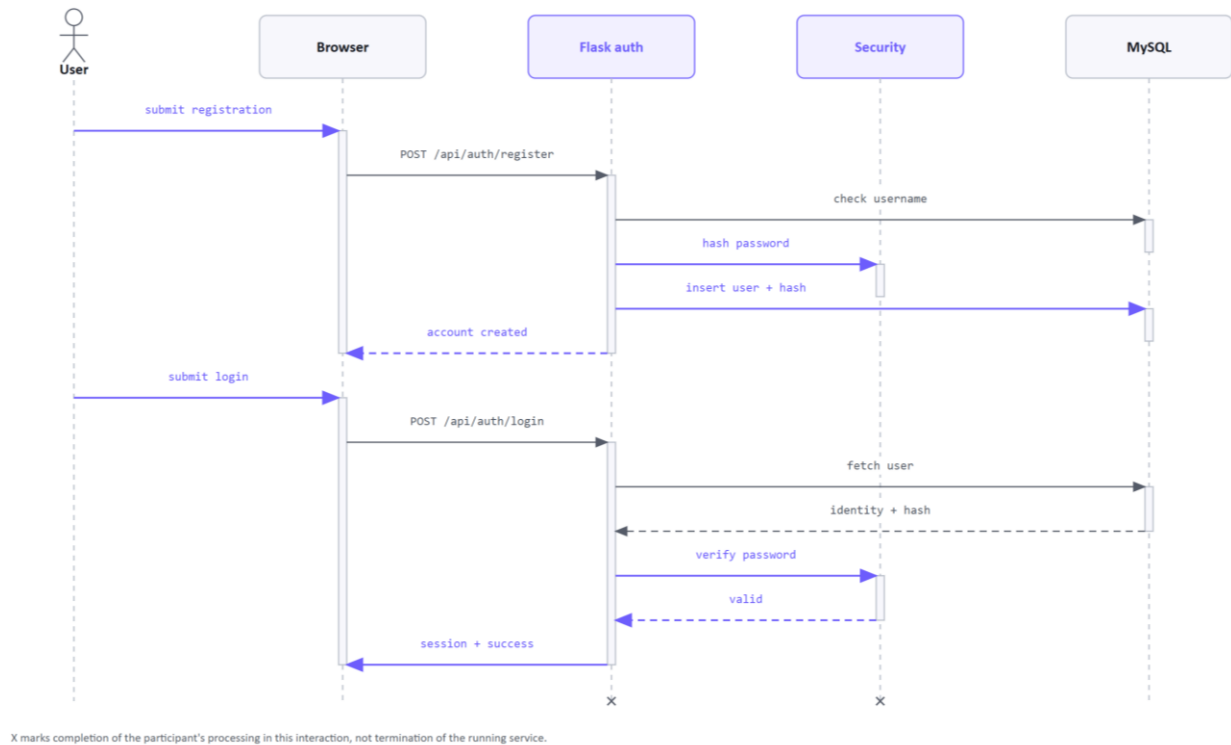
Figure 4.10-1: Authentication sequence.
