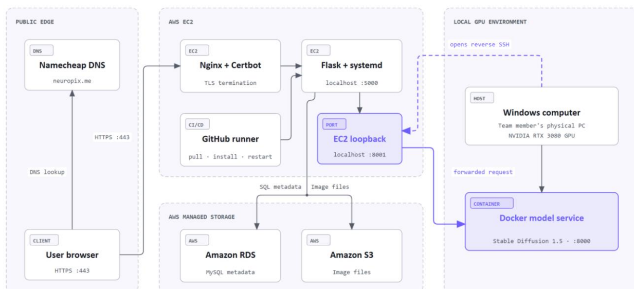
Figure 4.11: Production deployment and reverse SSH.
