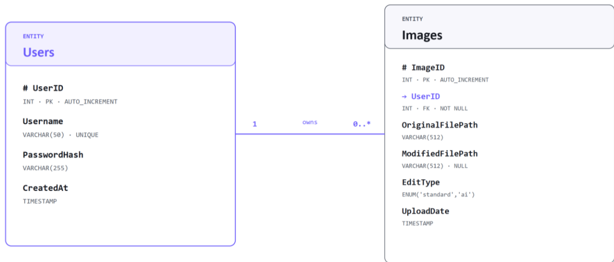
Figure 4.7: NeuroPix data model.
