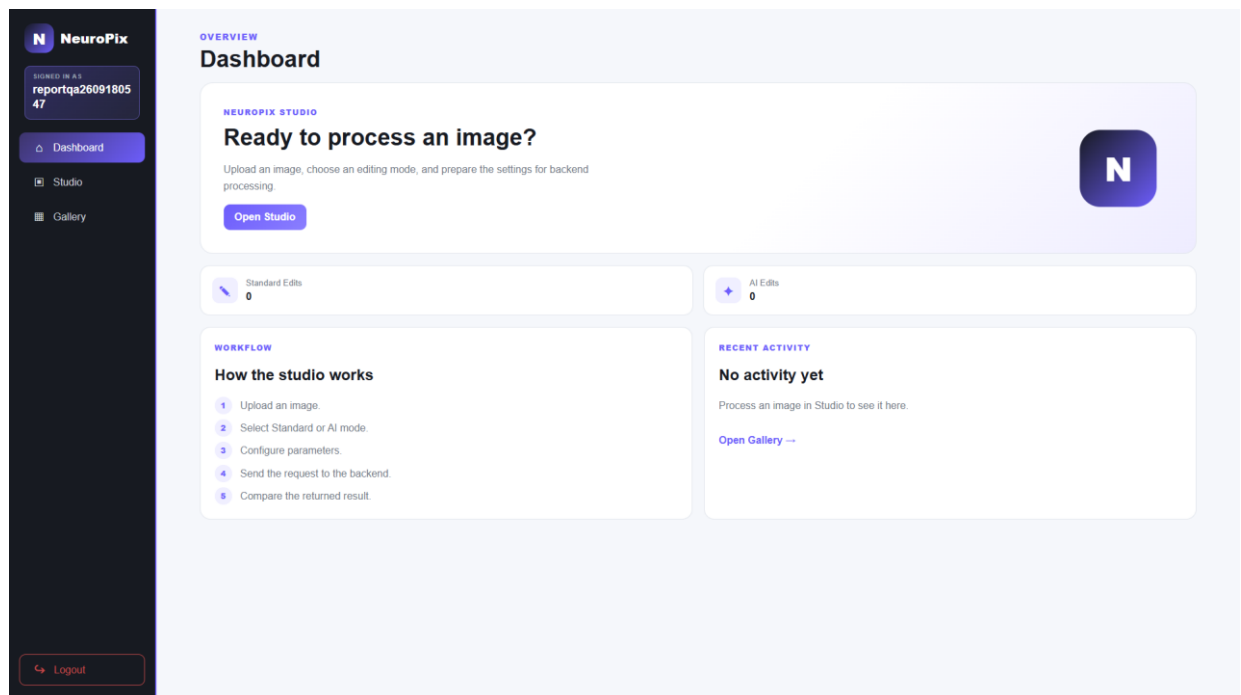
(a) Dashboard
