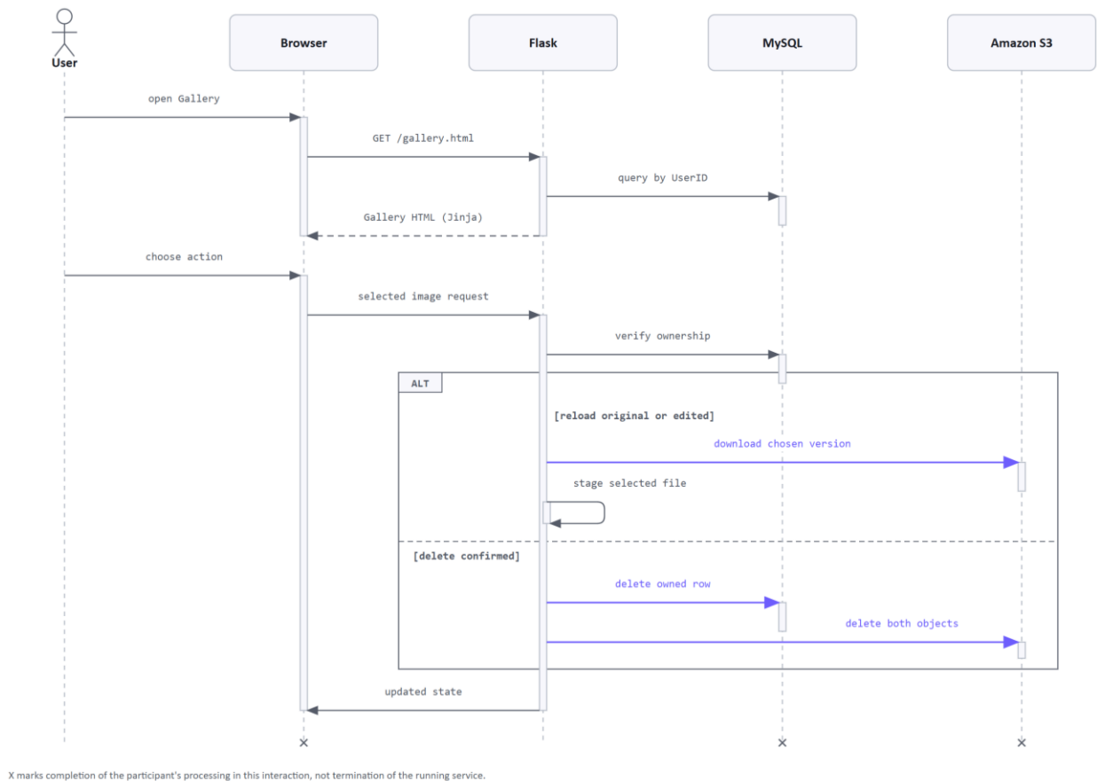
Figure 4.10-4: Gallery sequence.
