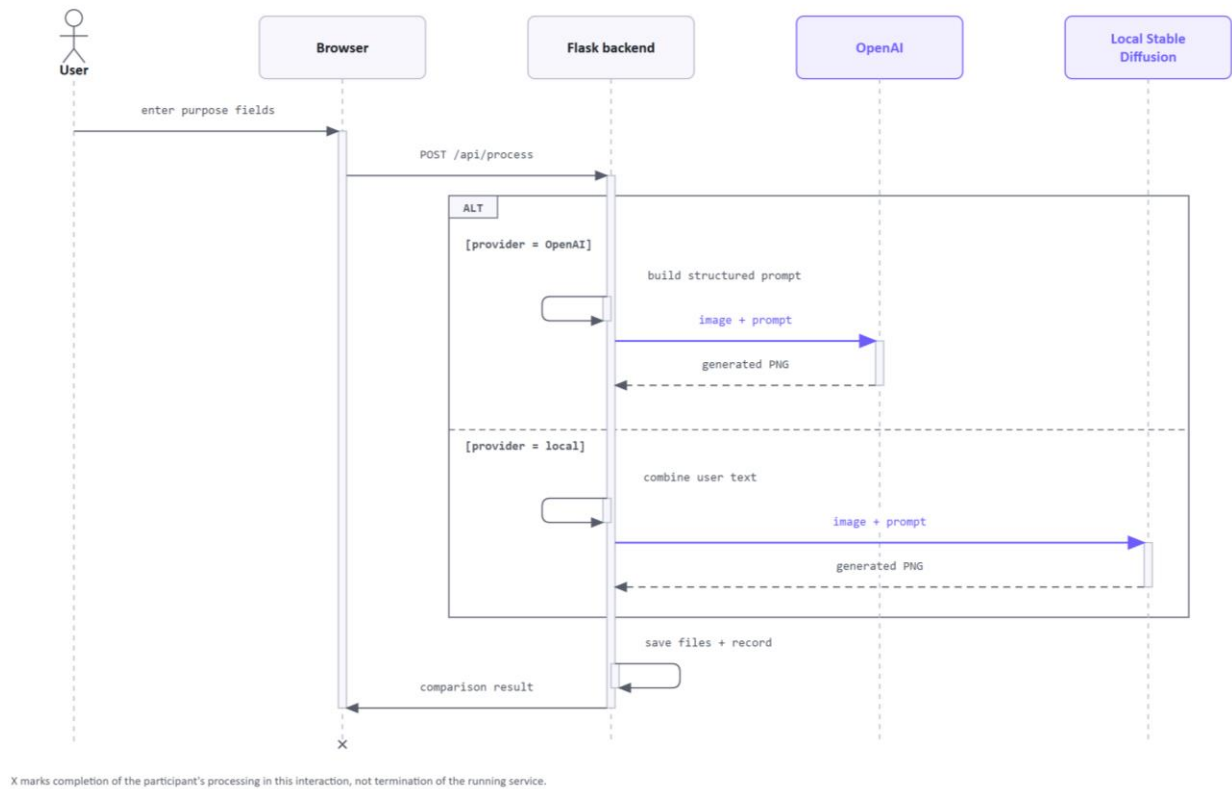
Figure 4.10-3: AI-provider sequence.
