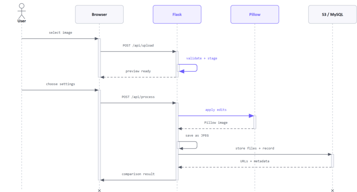
Figure 4.10-2: Standard-edit sequence.
