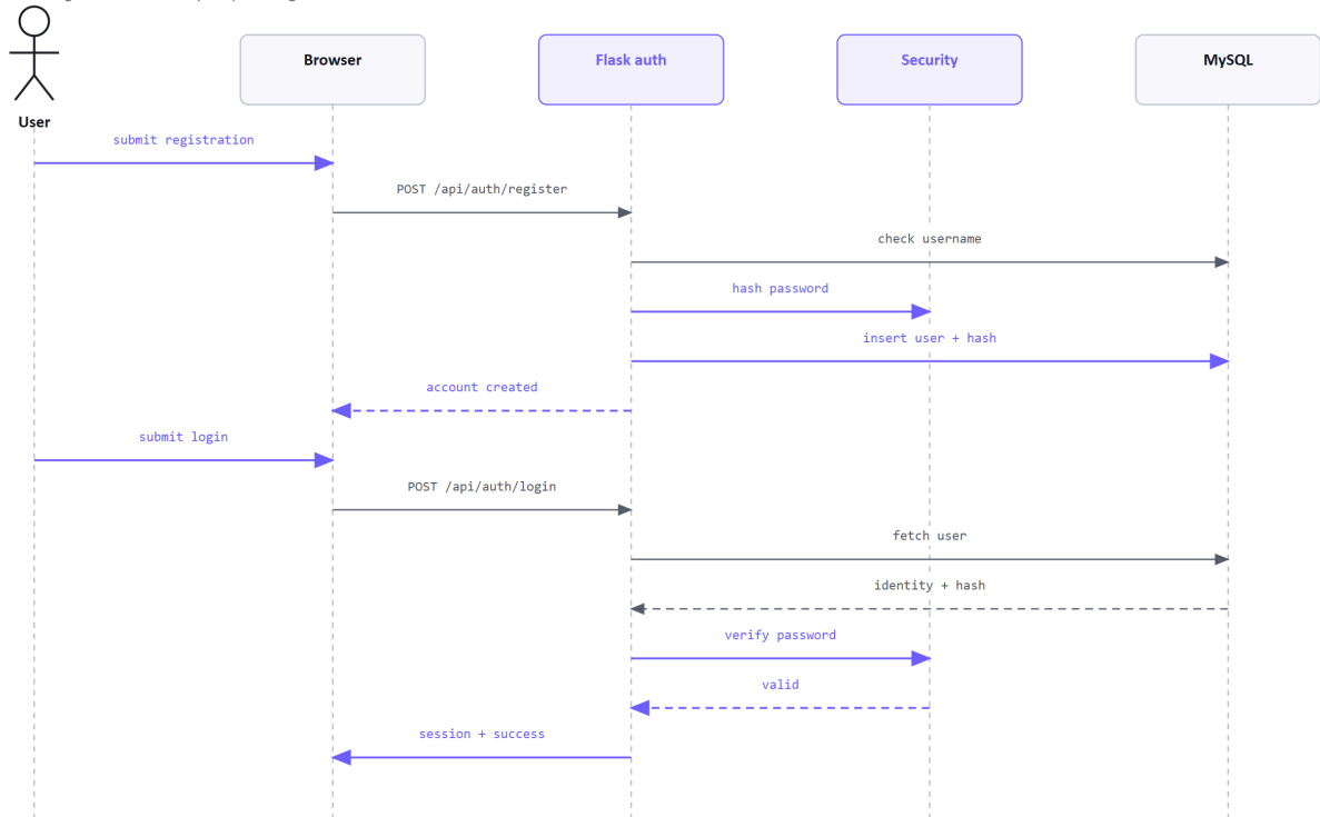
Figure 4.7: Authentication sequence.
