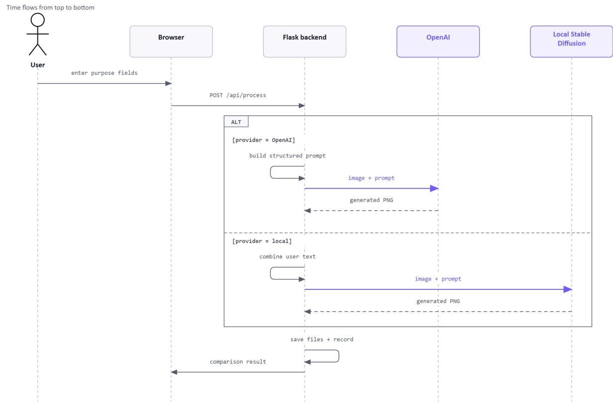
Figure 4.9: AI-provider sequence.
