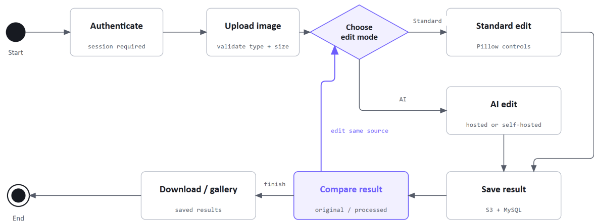
Figure 3.2: Authenticated editing activity.
