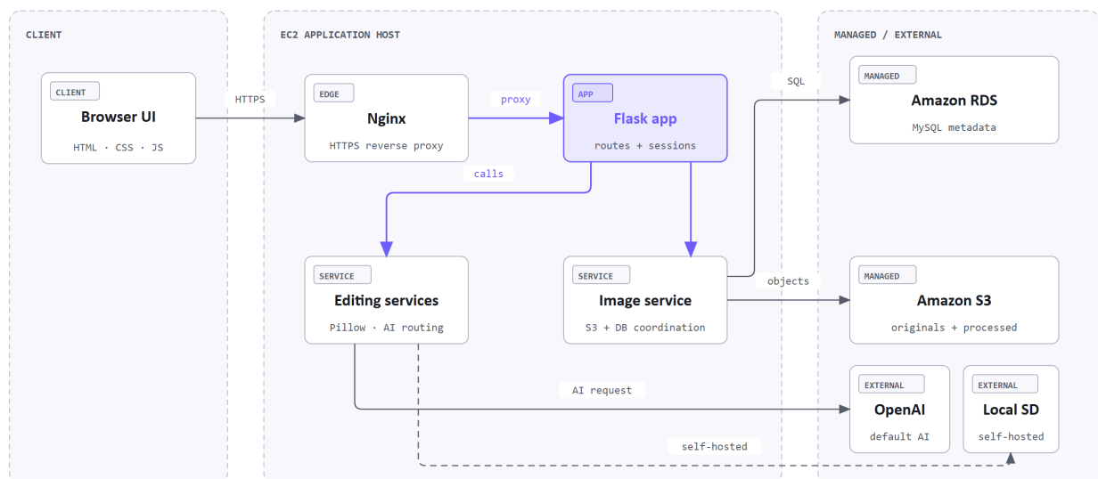
Figure 4.1: NeuroPix system architecture.
