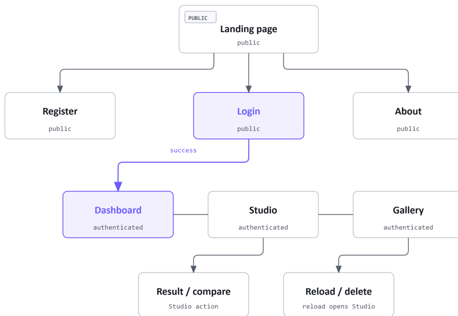
Figure 4.2: Frontend navigation and access.
