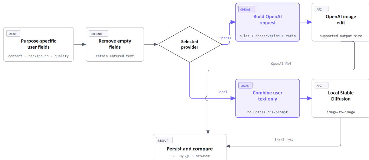
Figure 4.4: AI prompt and provider routing.
