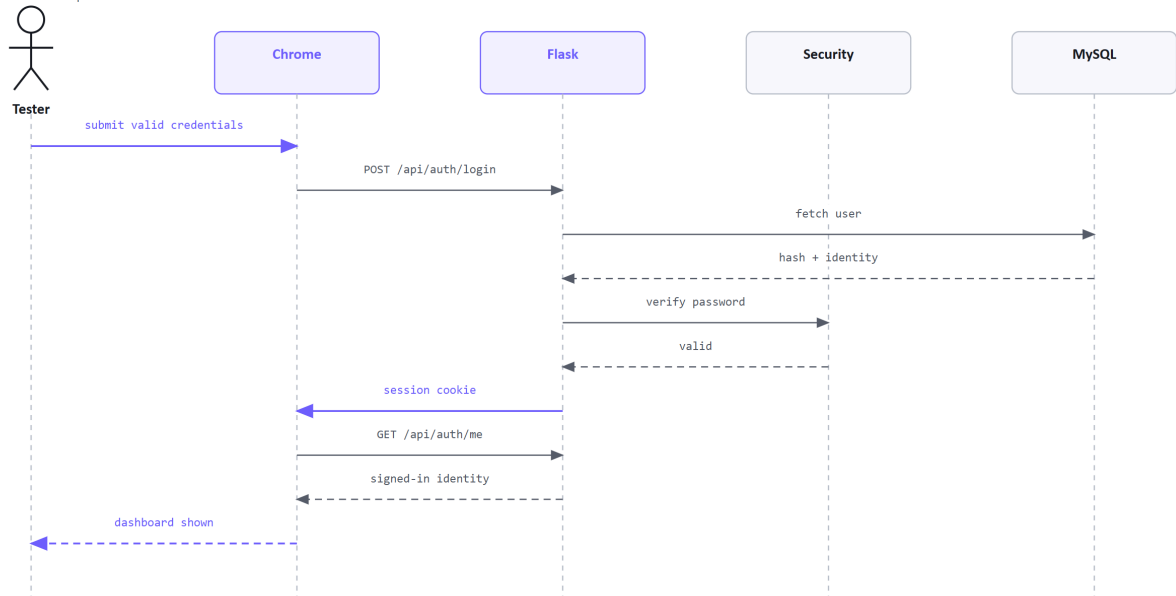
Figure 6.3: UC-T02 login and protected-access sequence.
