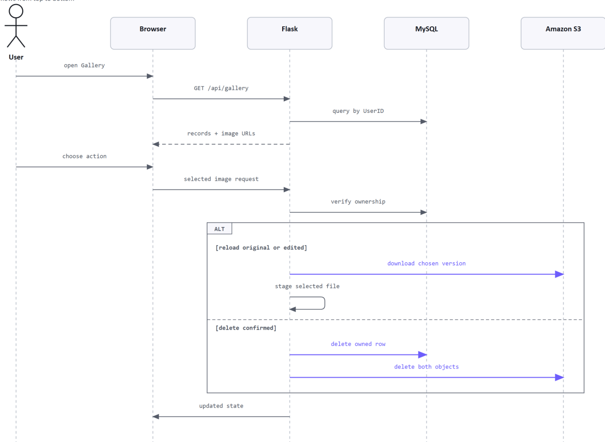
Figure 4.10: Gallery sequence.
