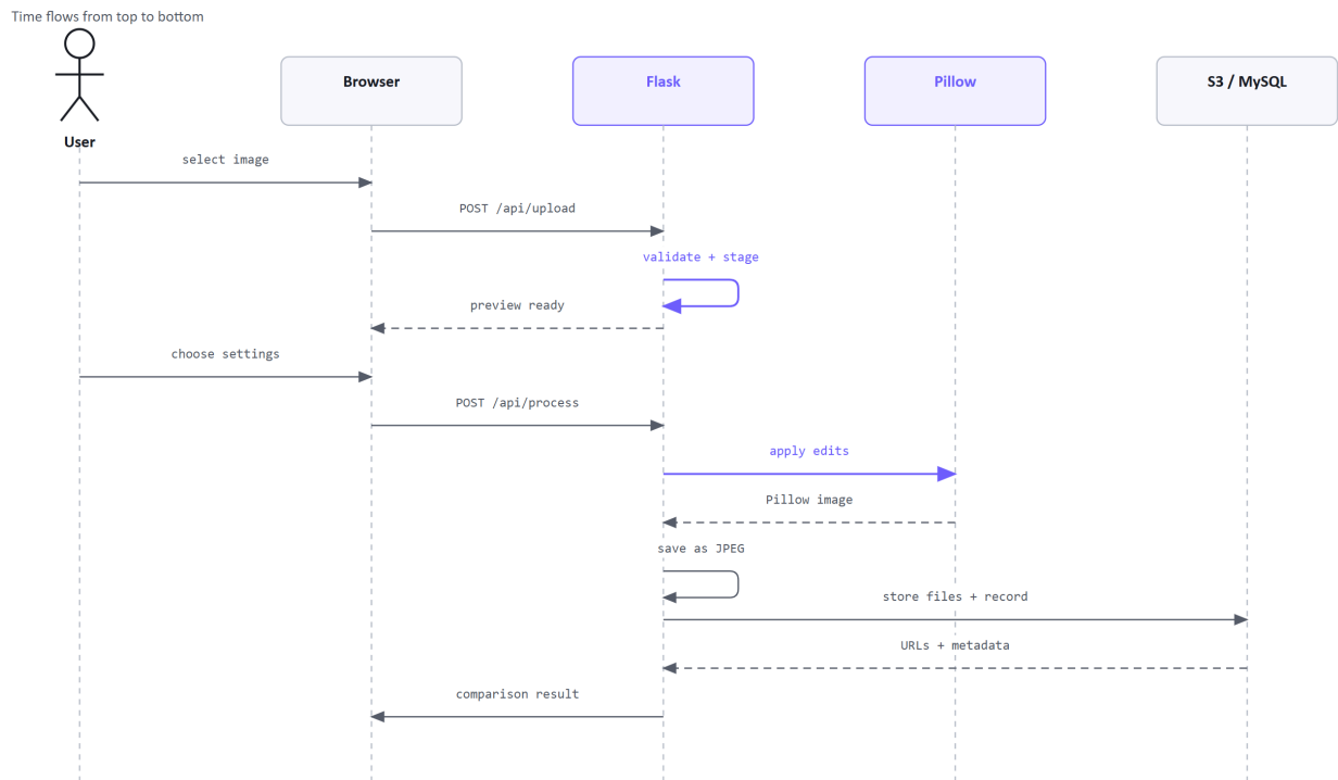
Figure 4.8: Standard-edit sequence.
