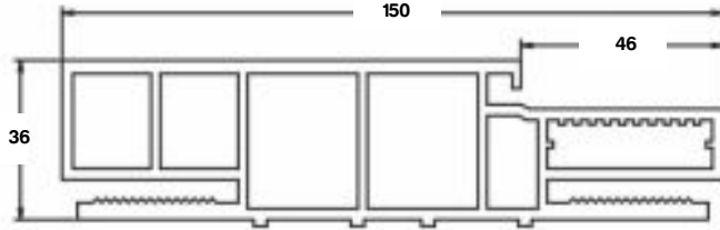
150 PVC FRAME PROFILE
