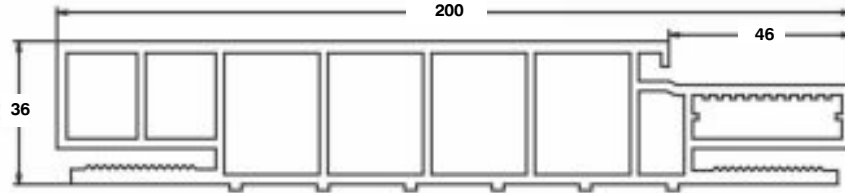
200 PVC FRAME PROFILE
