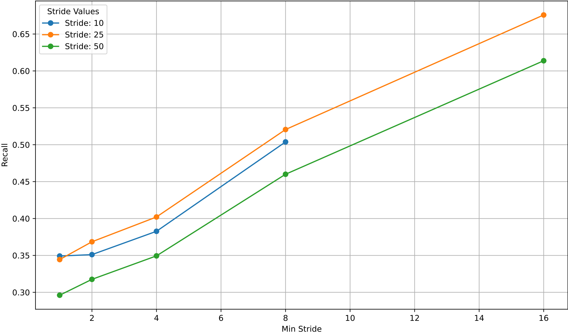
Recall over Min Stride for nprobe-10.csv (by Stride)
