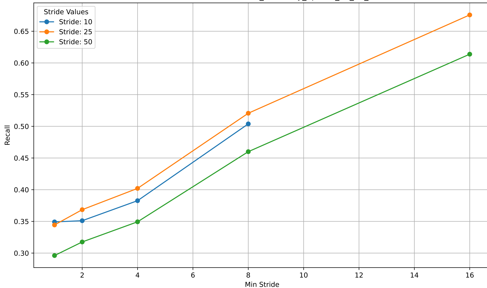
Recall over Min Stride for bsivf_summary_nprobe_10_tol_0.csv
