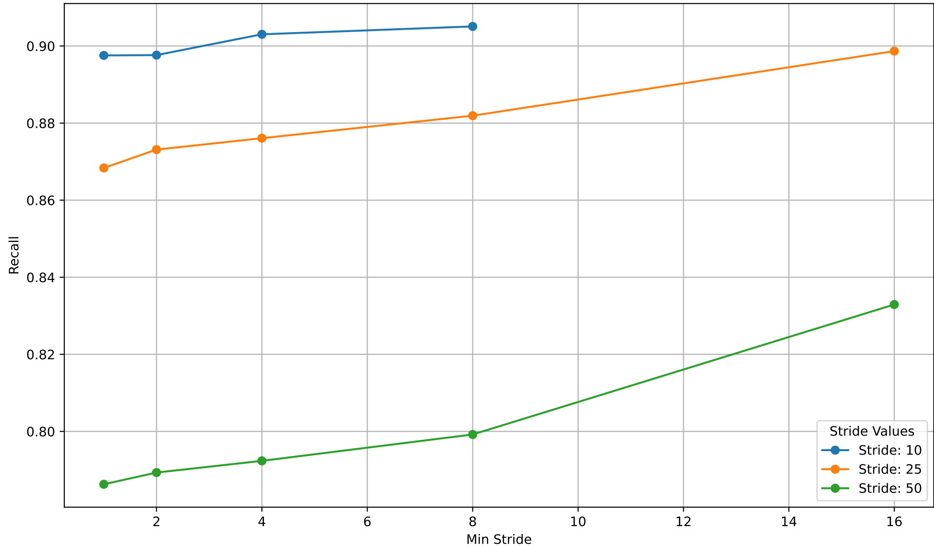
Recall over Min Stride for bsivf_summary_nprobe_10_tol_10.csv
