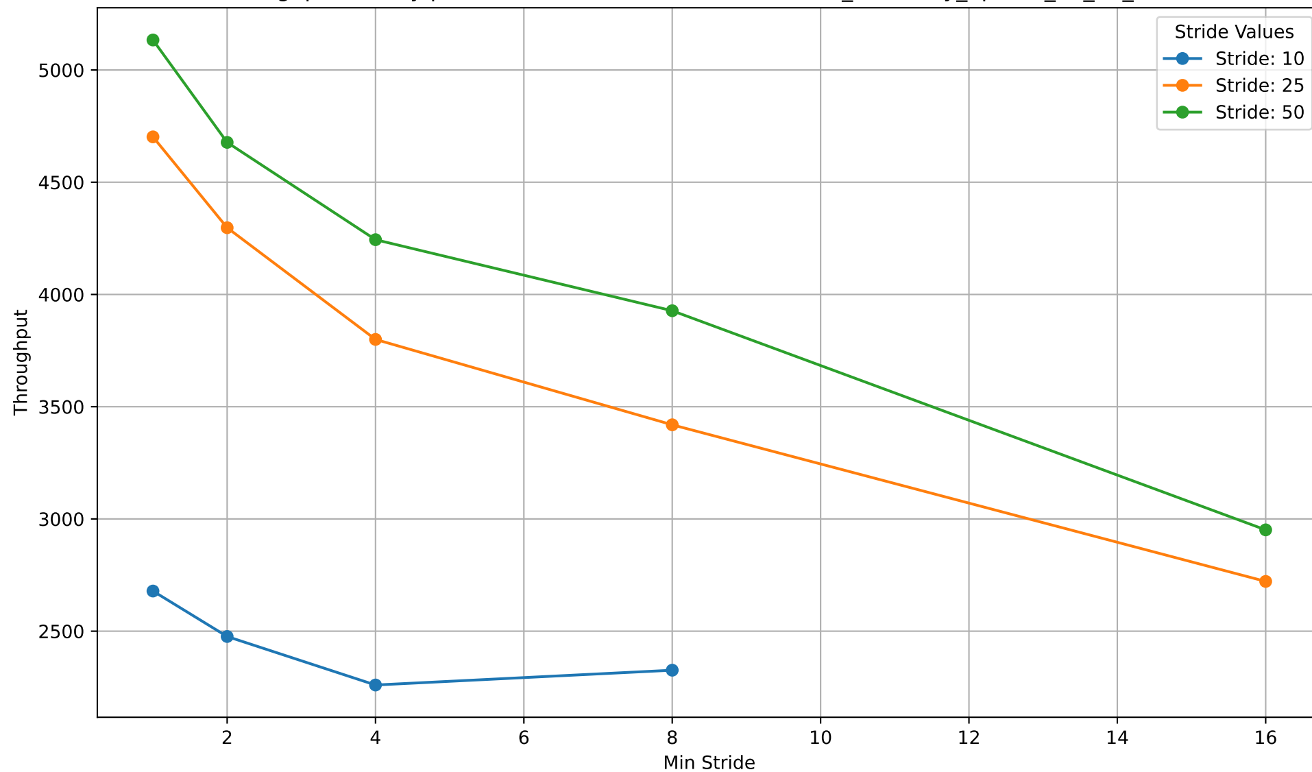
Throughput (Query per seconds) over Min Stride for bsivf_summary_nprobe_10_tol_10.csv
