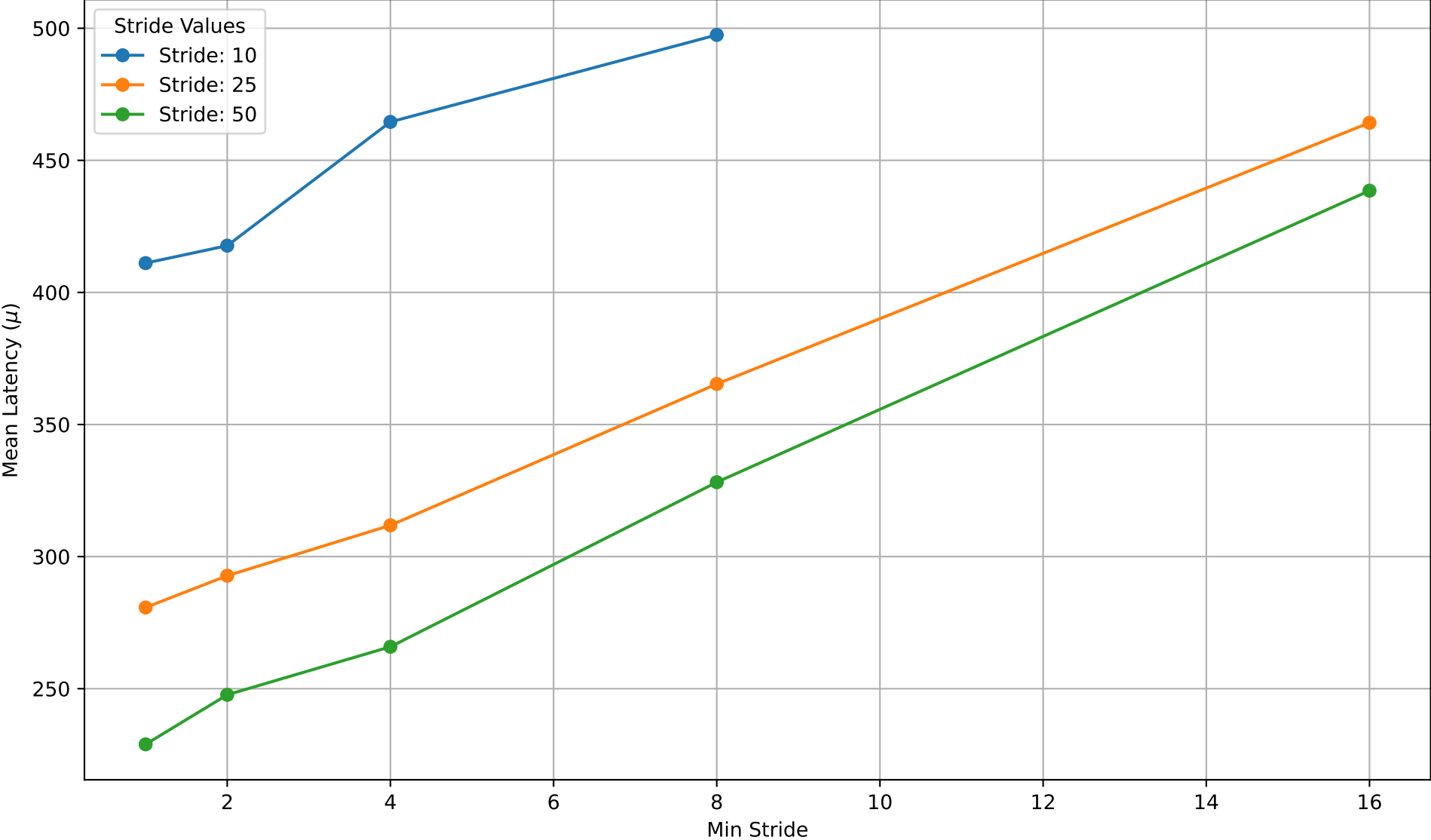
Mean latency ( \mu s) over Min Stride for bsivf_summary_nprobe_15_tol_0.csv
