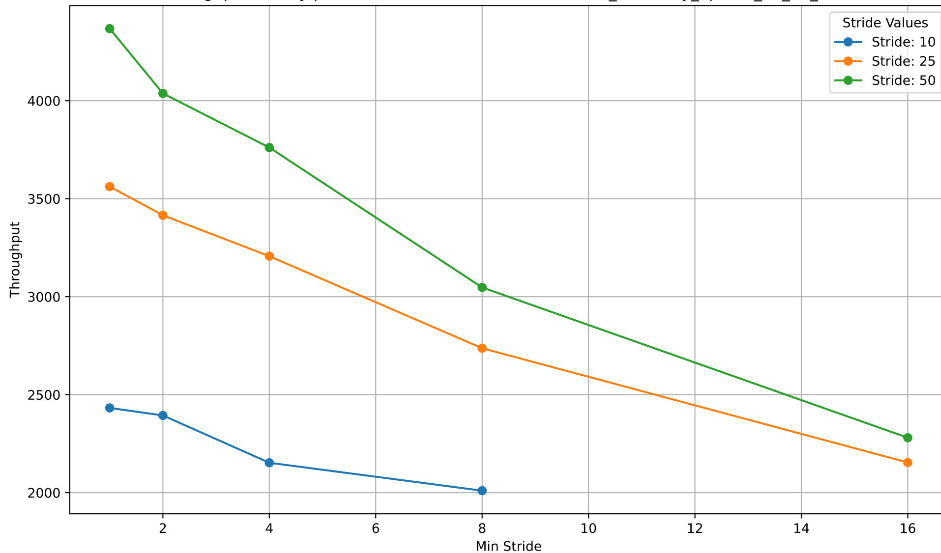
Throughput (Query per seconds) over Min Stride for bsivf_summary_nprobe_15_tol_0.csv
