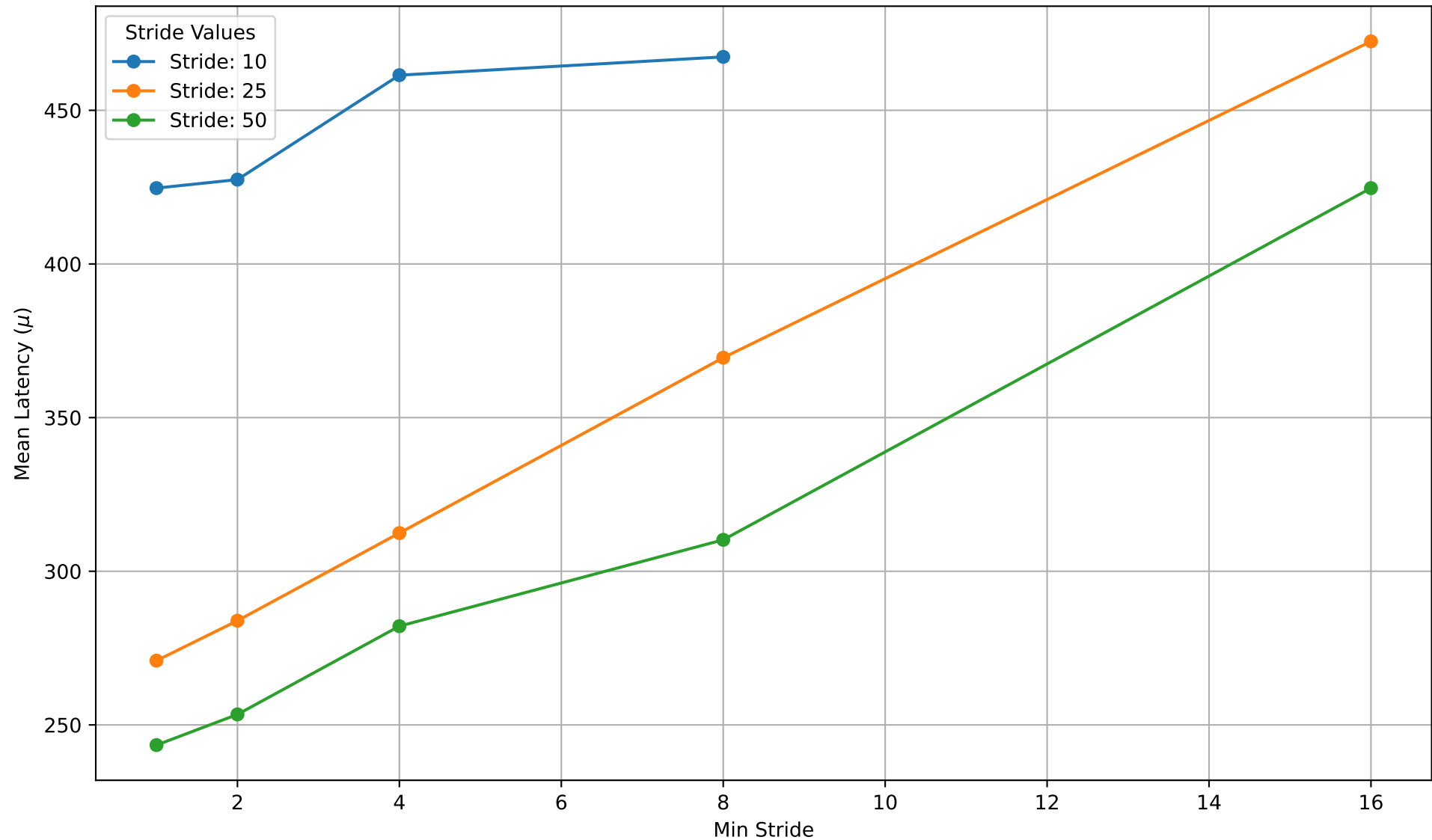
Mean latency ( \mu s) over Min Stride for bsivf_summary_nprobe_15_tol_10.csv
