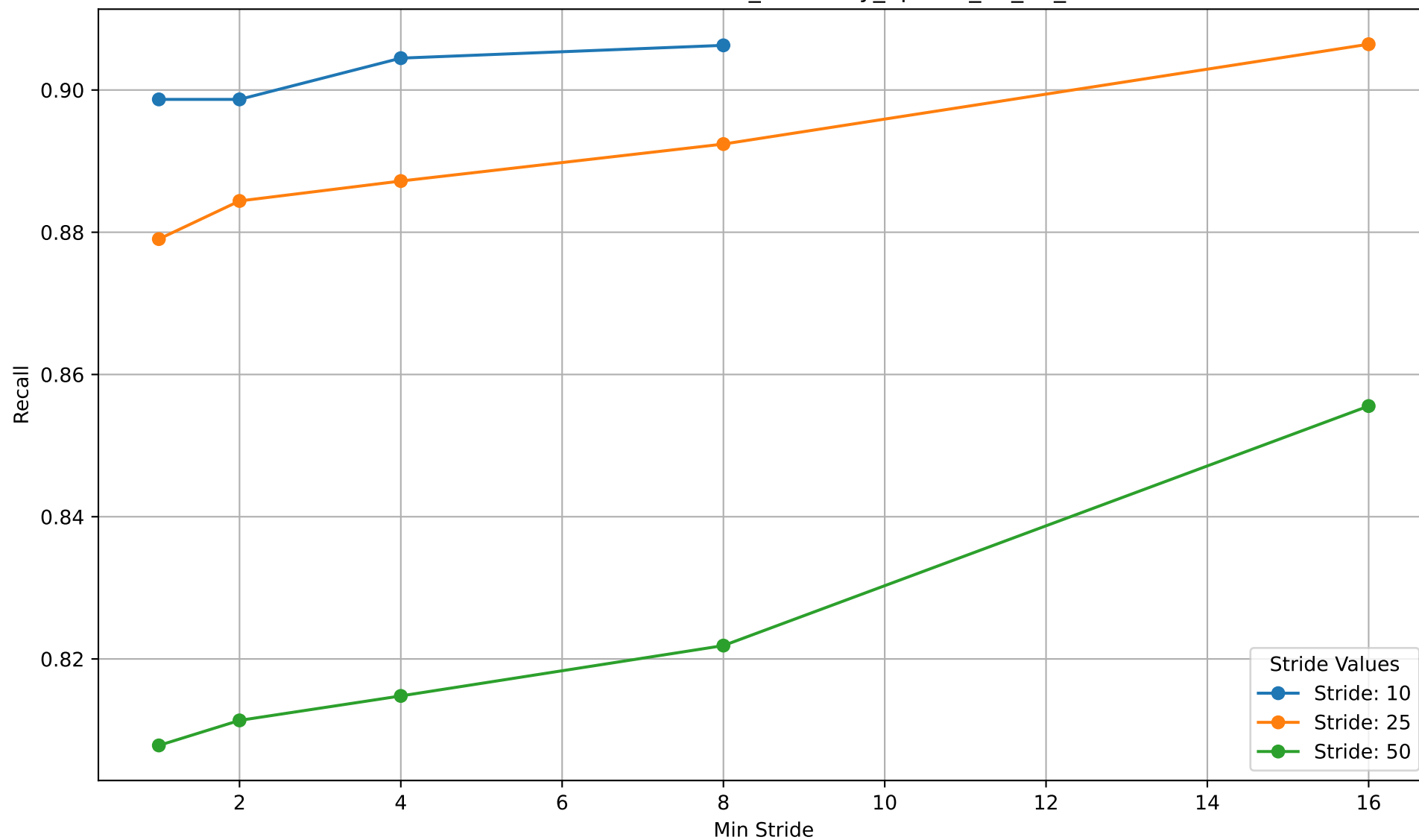
Recall over Min Stride for bsivf_summary_nprobe_15_tol_10.csv
