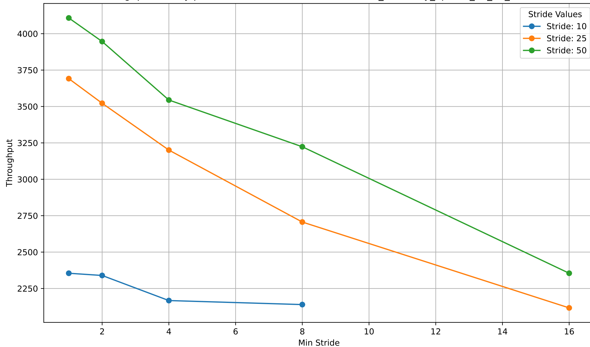
Throughput (Query per seconds) over Min Stride for bsivf_summary_nprobe_15_tol_10.csv
