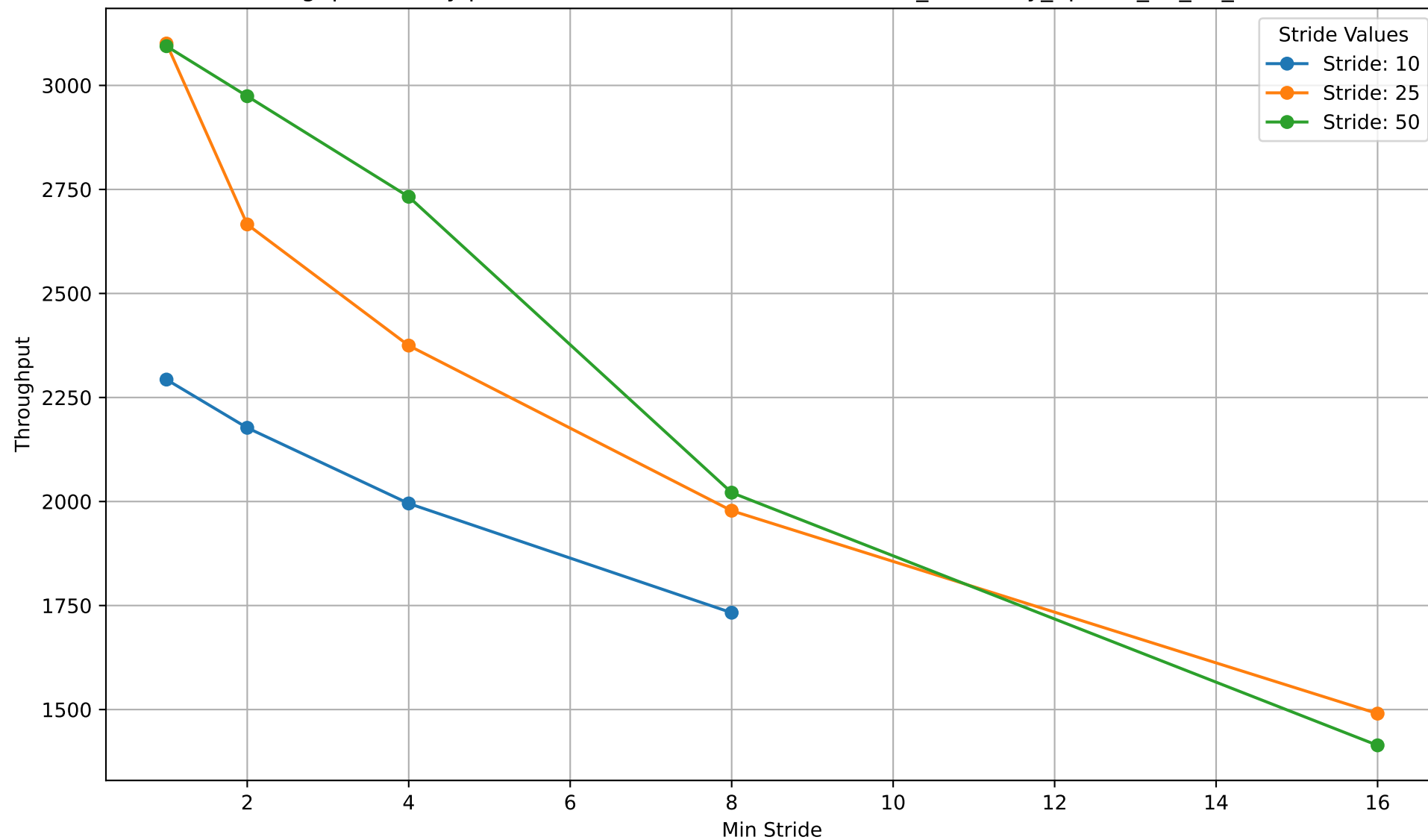
Throughput (Query per seconds) over Min Stride for bsivf_summary_nprobe_25_tol_10.csv
