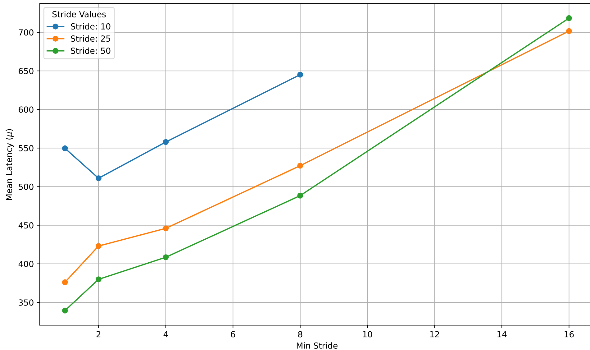
Mean latency ( \mu s) over Min Stride for bsivf_summary_nprobe_tol_by_stride.csv
