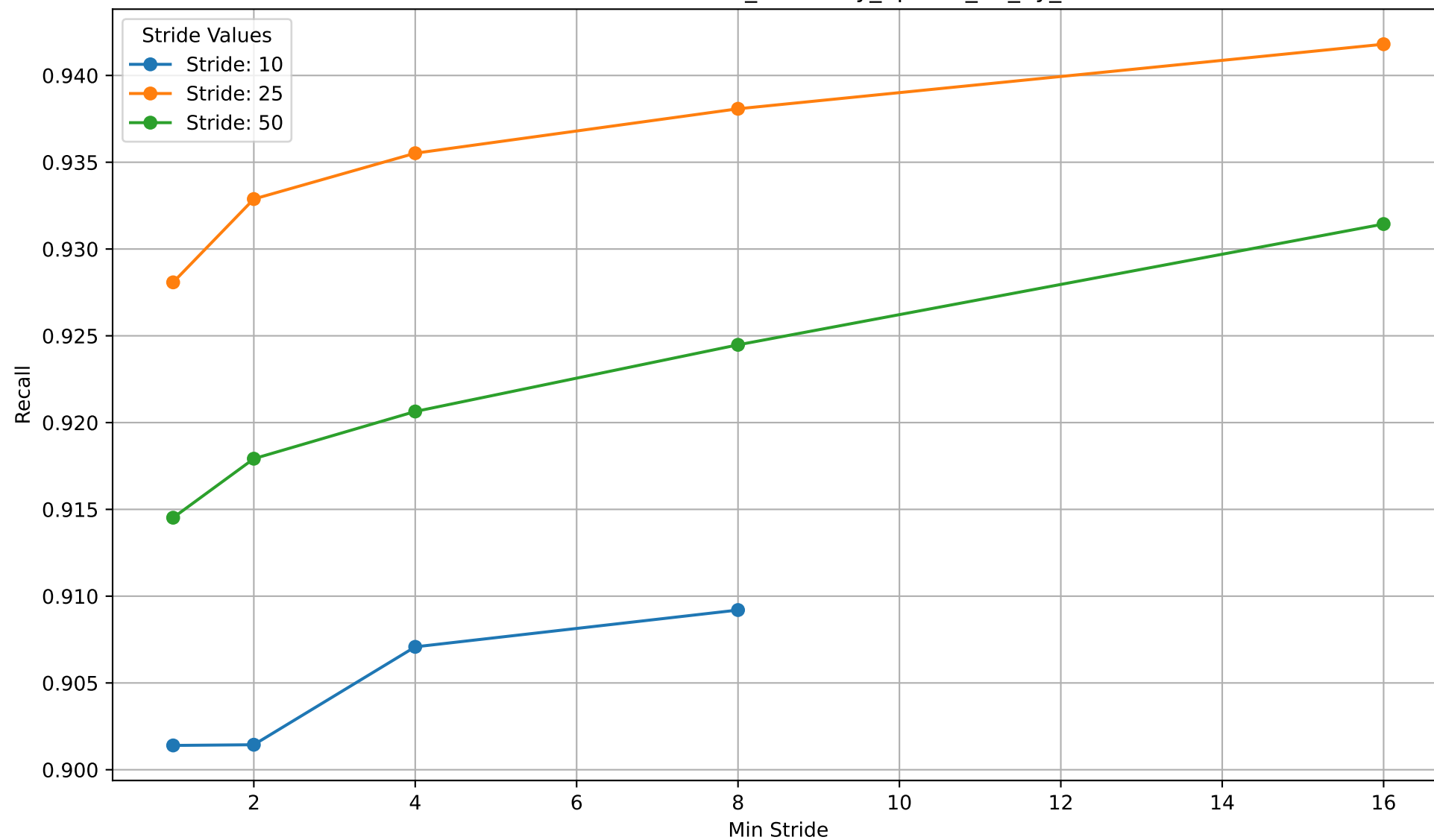
Recall over Min Stride for bsivf_summary_nprobe_tol_by_stride.csv
