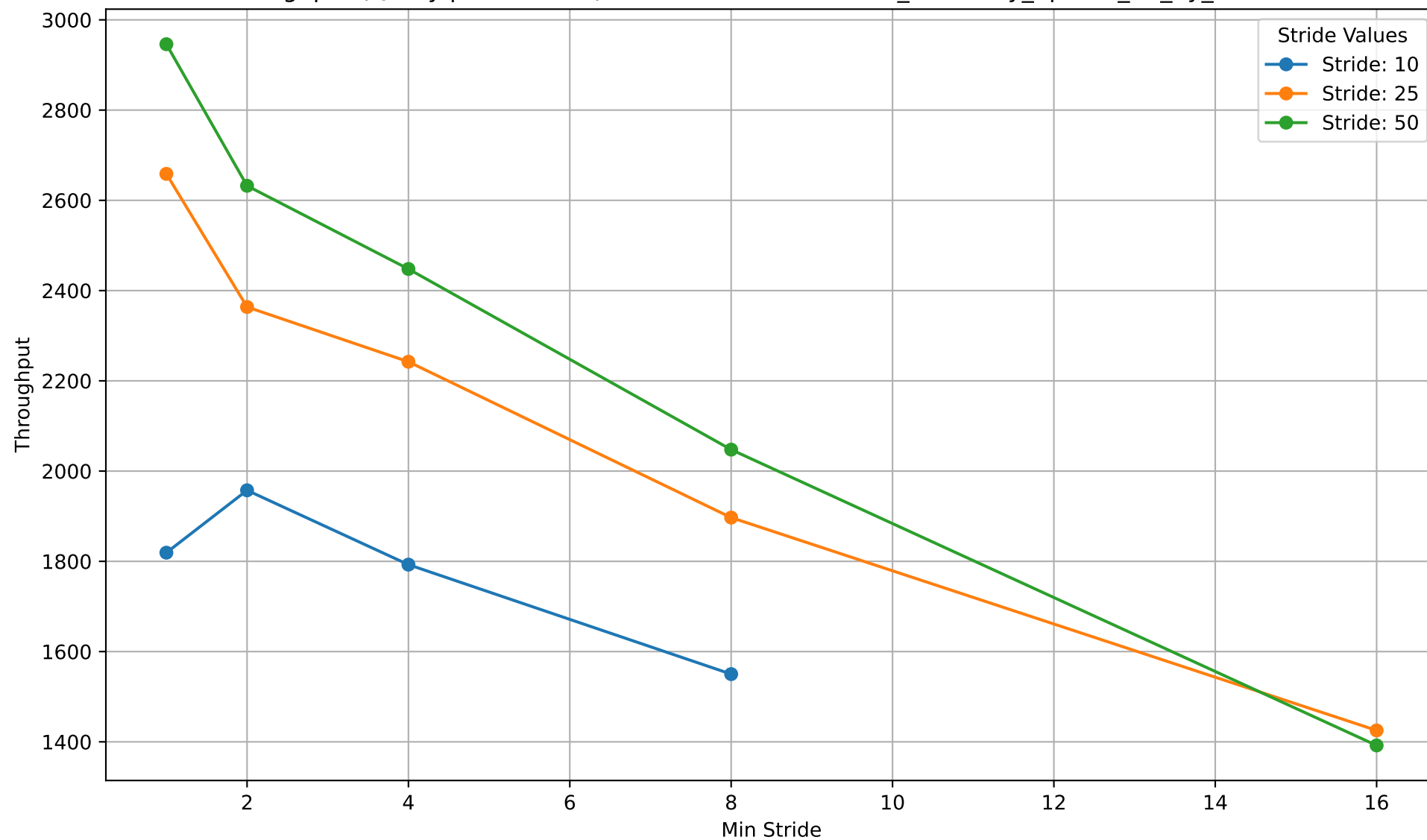
Throughput (Query per seconds) over Min Stride for bsivf_summary_nprobe_tol_by_stride.csv
