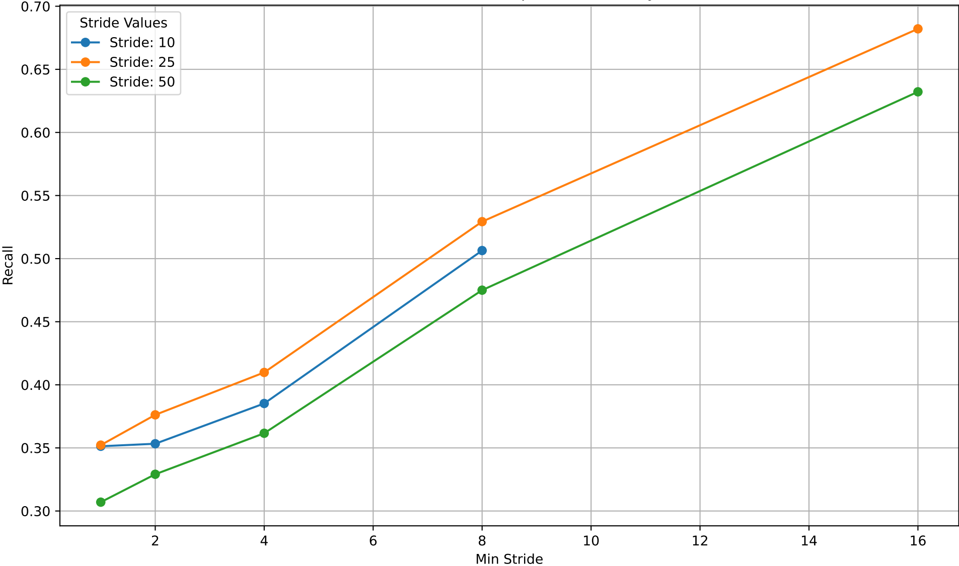
Recall over Min Stride for nprobe-15.csv (by Stride)
