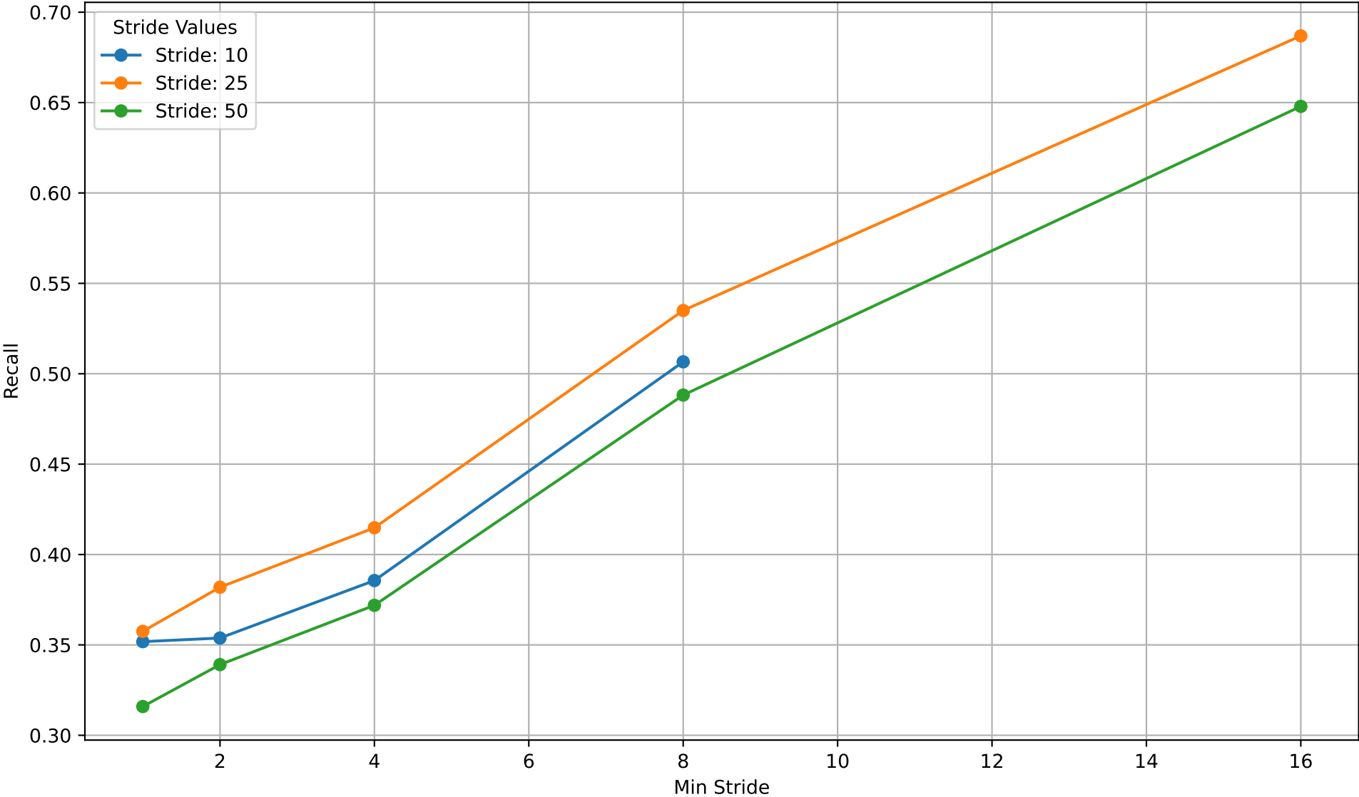
Recall over Min Stride for nprobe-25.csv (by Stride)
