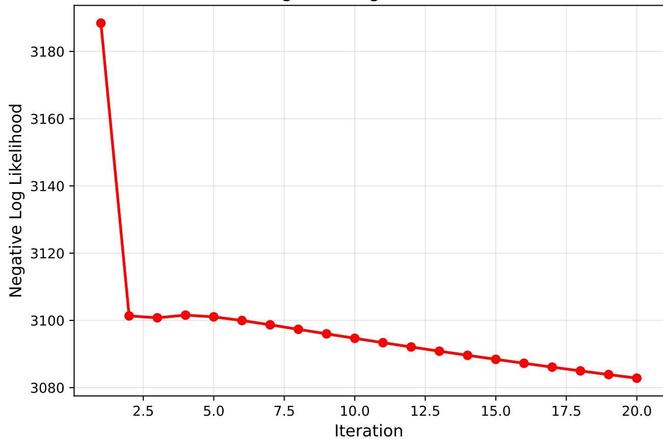
Negative Log Likelihood
