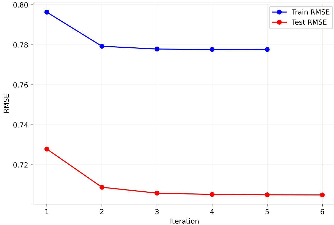
RMSE
