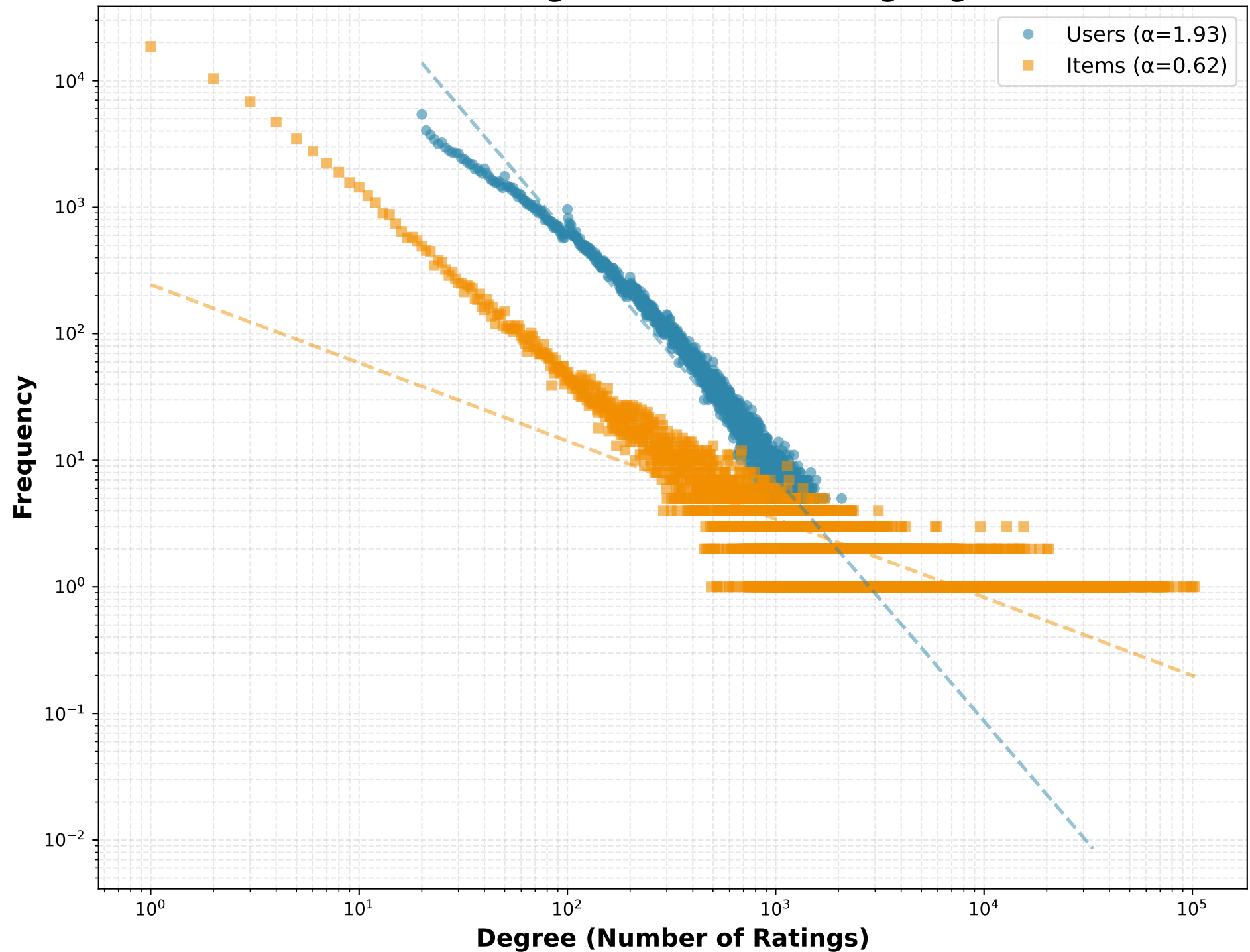
User and Item Degree Distribution (Log-Log Scale)
