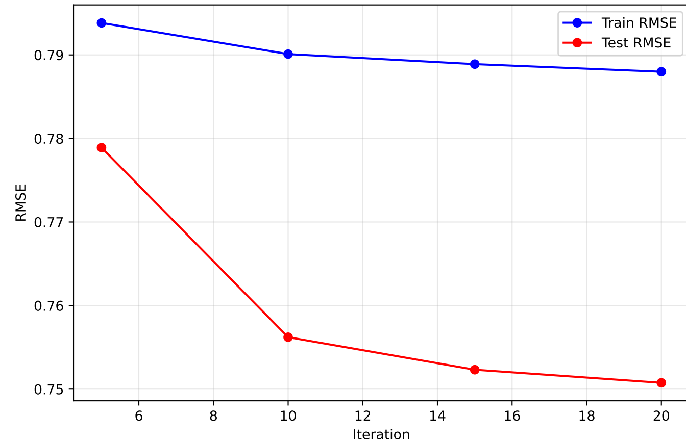
RMSE
