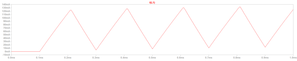
Şekil 3.11: Current waveform for the 10 mH – 10 Ω coil
