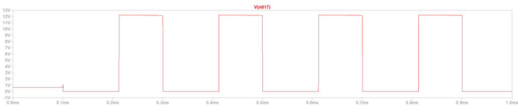
Şekil 3.13: V2 voltage waveform for the 10 mH – 10 Ω coil
