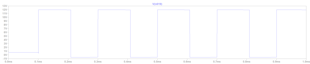
Şekil 3.12: V1 voltage waveform for the 10 mH – 10 Ω coil
