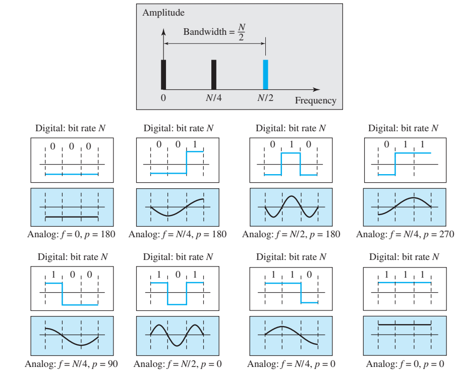
Figure 3.22 Rough approximation of a digital signal using the first harmonic for worst case
