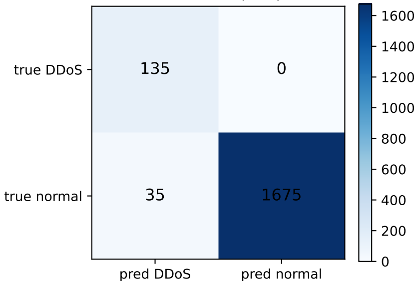
Confusion (test)
