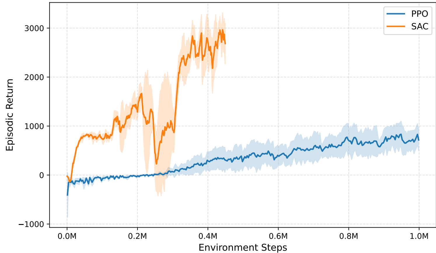
PPO vs SAC — Ant-v4
