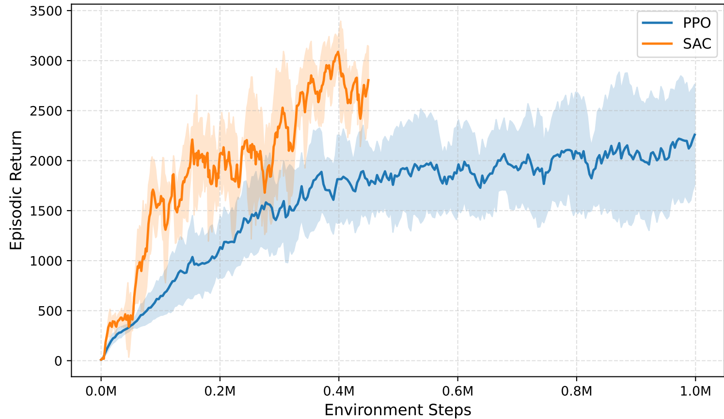
PPO vs SAC — Hopper-v4
