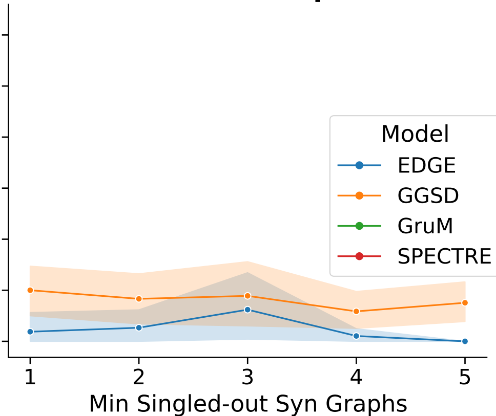
Dataset: Elliptic
