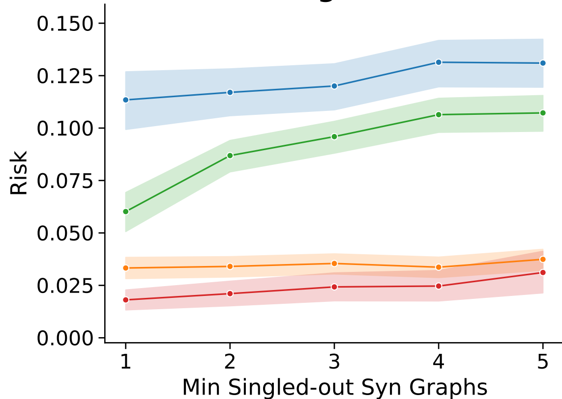
Dataset: Ego-Facebook
